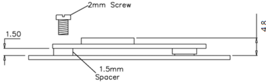
Figure 7: Mounting information for MSD50NB
