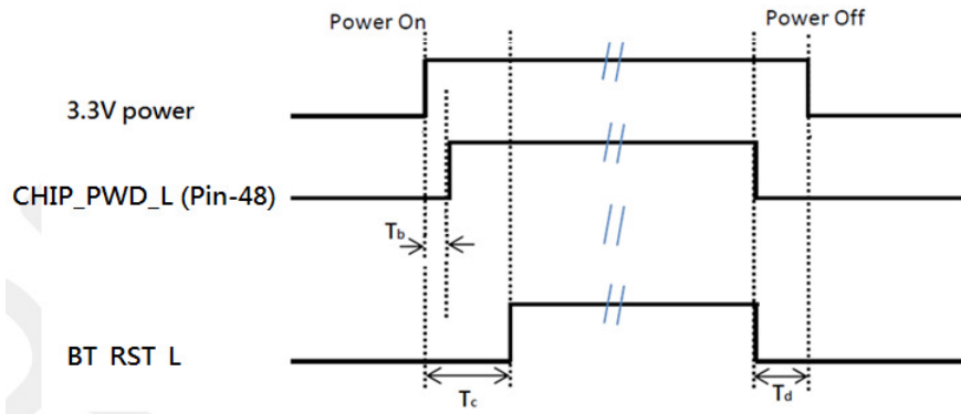
Figure 1: Power On/Off Timing
