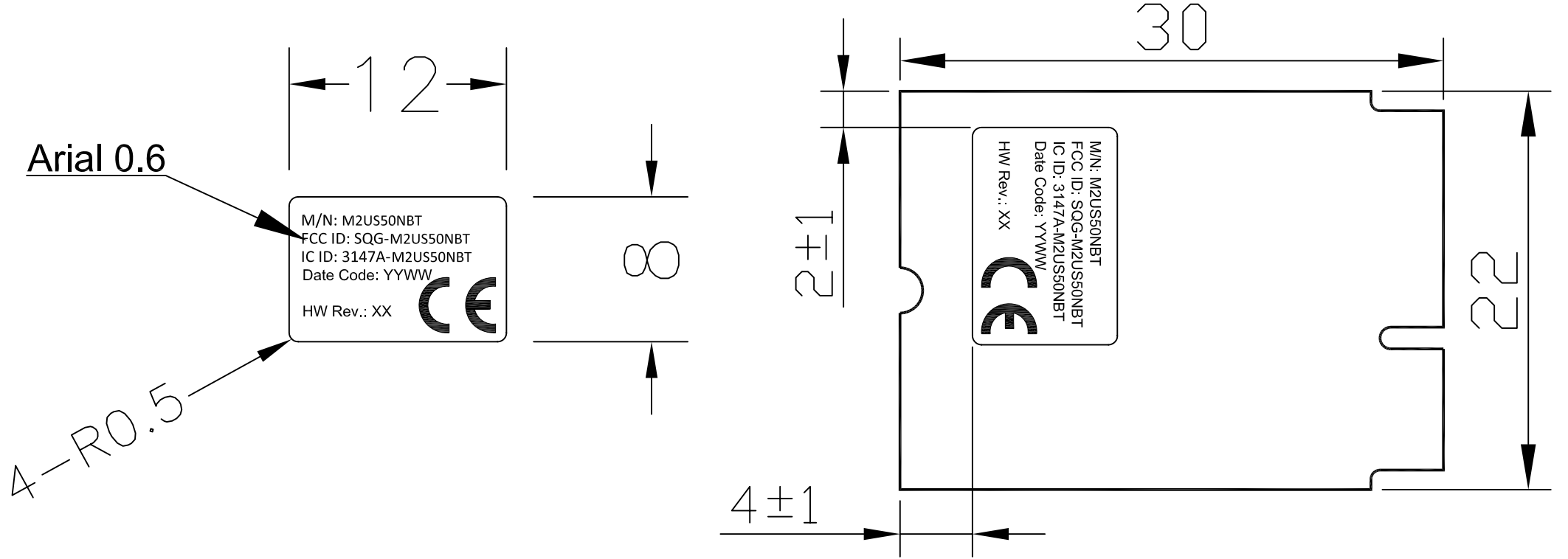
Label on PCBA back
