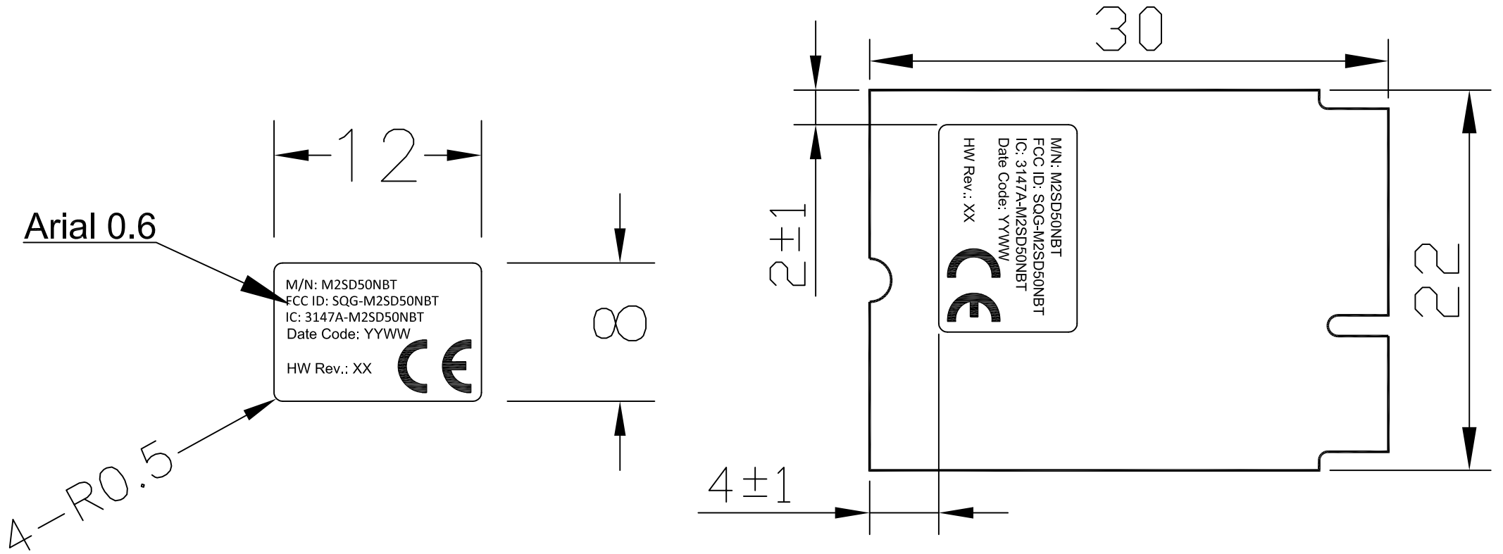
Label on PCBA back
