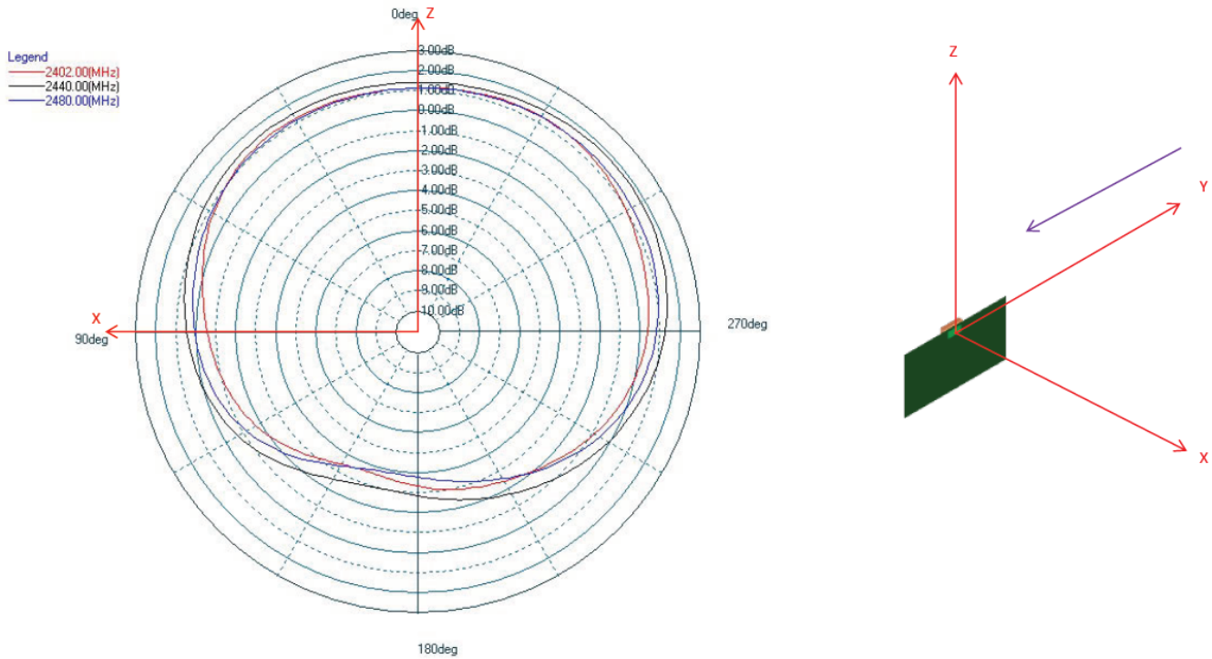
Typical 2D Antenna Radiation Patterns - Phi 0° (Side View) Gain (dBi)
