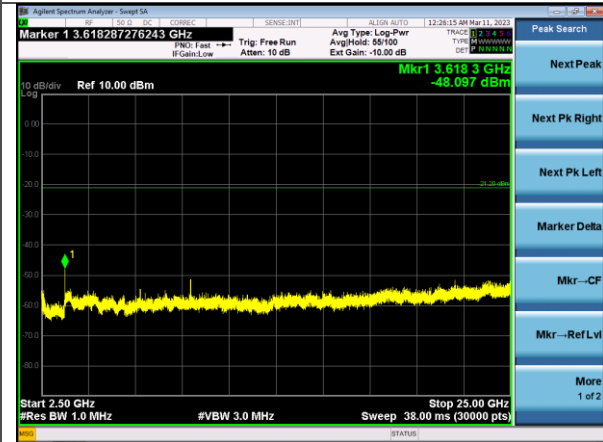
2.5-25 GHz Peak Ch 1
