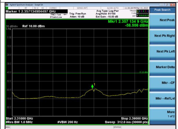
2.31-2.39 GHz Average Ch 11
