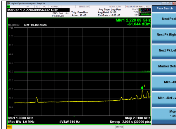
1-2.31 GHz Average Ch 6
