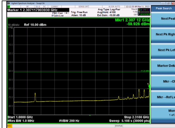
1-2.31 GHz Average Ch 1
