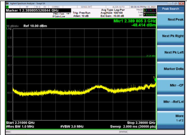
2.31-2.39 GHz Peak Ch 11
