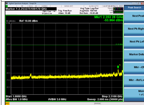
1-2.31 GHz Peak Ch 11
