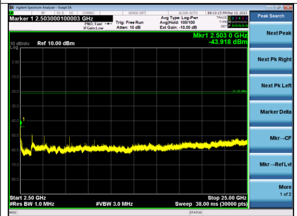
2.5-25 GHz Peak Ch 11
