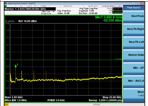
2.5-25 GHz Average Ch 6
