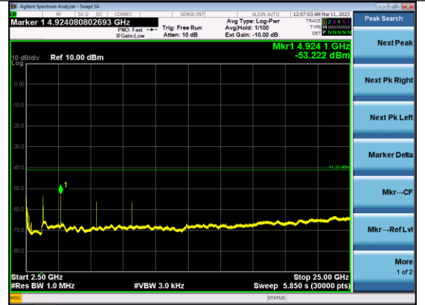
2.5-25 GHz Average Ch 11
