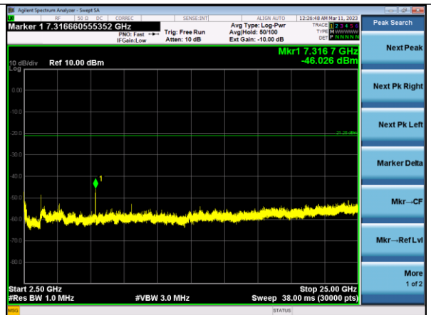
2.5-25 GHz Peak Ch 6
