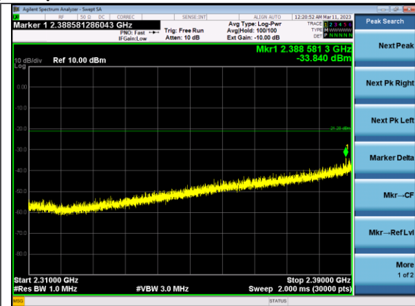
2.31-2.39 GHz Peak Ch 1
