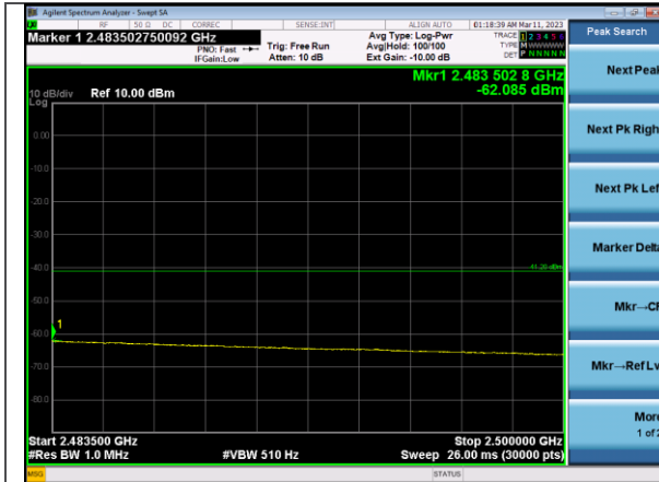
2.4835-2.5 GHz Average Ch 1
