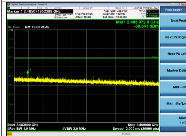
2.4835-2.5 GHz Peak Ch 6
