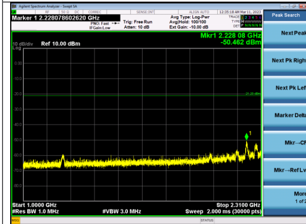
1-2.31 GHz Peak Ch 6
