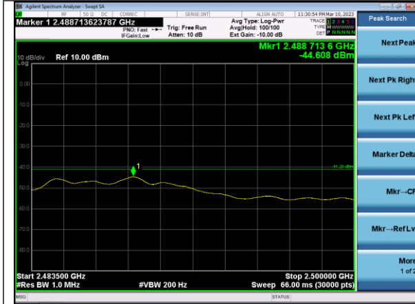
2.4835-2.5 GHz Average Ch 11
