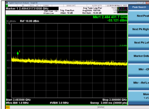
2.4835-2.5 GHz Peak Ch 11
