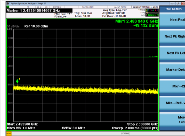
2.4835-2.5 GHz Peak Ch 1
