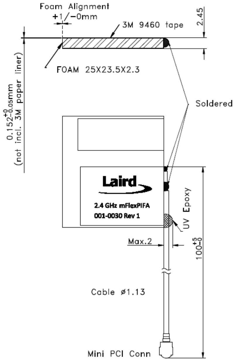
Figure 1: Physical dimensions
