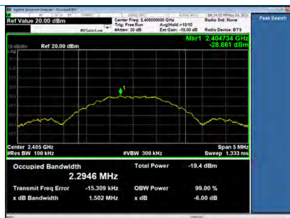
DTS BW, Channel 11, neg40dBm
