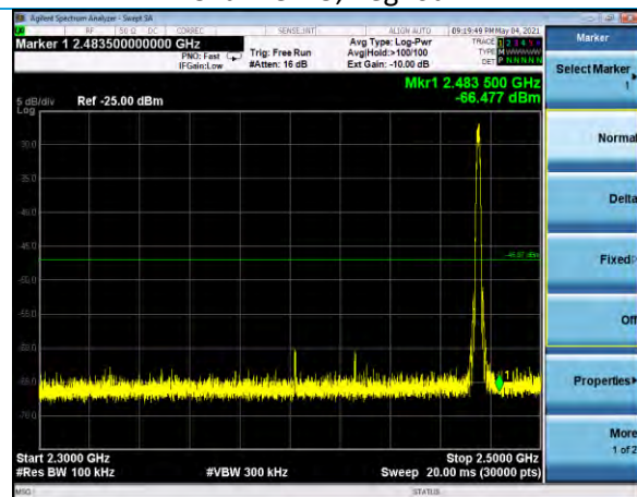
Conducted TX Spurious 2.3-2.5 GHz Channel 25, neg40dBm
