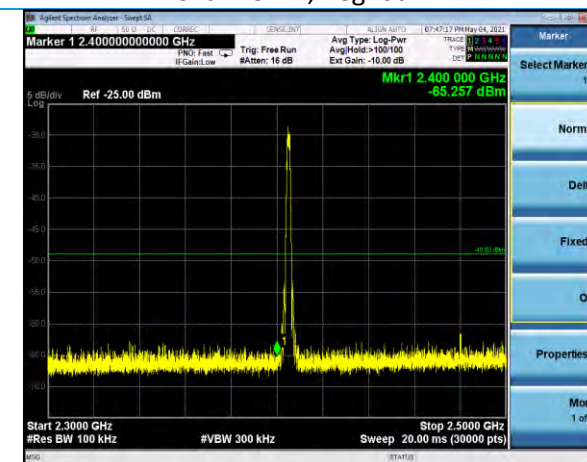
Conducted TX Spurious 2.3-2.5 GHz Channel 11, neg40dBm
