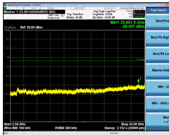
Conducted TX Spurious 2.5-25 GHz Channel 19, neg4dBm
