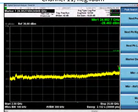
Conducted TX Spurious 2.5-25 GHz Channel 11, neg4dBm
