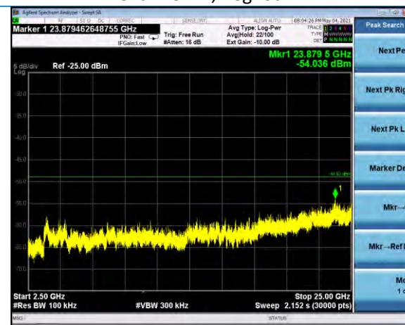
Conducted TX Spurious 2.5-25 GHz Channel 11, neg40dBm
