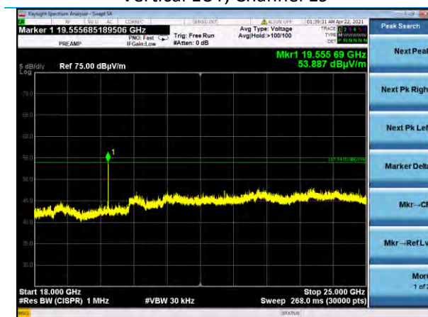
18-25 GHz, Horizontal Antenna Vertical EUT, Channel 19
