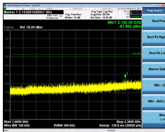
Conducted TX Spurious 1-2.3 GHz Channel 11, neg4dBm
