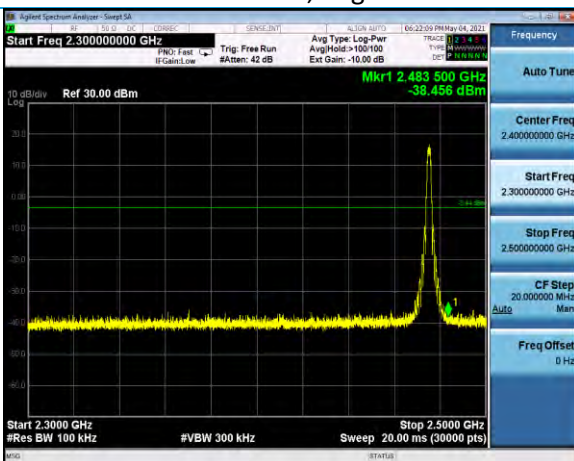
Conducted TX Spurious 2.3-2.5 GHz Channel 25, neg4dBm
