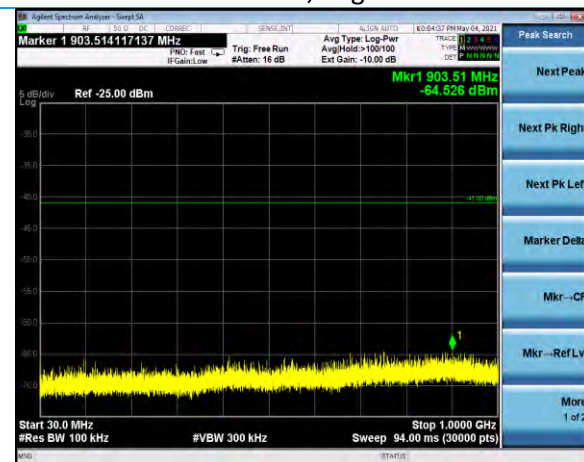
Conducted TX Spurious 30-1000 MHz Channel 25, neg4dBm
