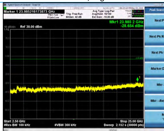
Conducted TX Spurious 2.5-25 GHz Channel 25, neg4dBm
