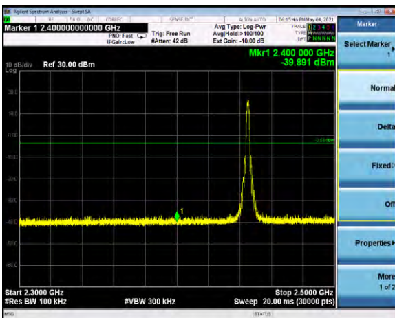
Conducted TX Spurious 2.3-2.5 GHz Channel 19, neg4dBm
