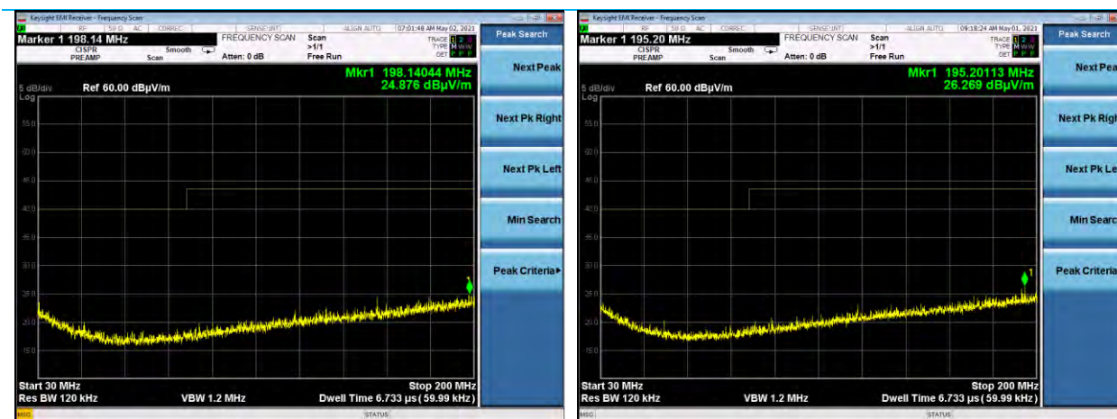
30-200 MHz, Horizontal Antenna Vertical EUT, Channel 19
