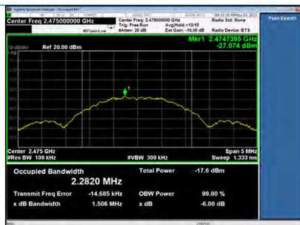
DTS BW, Channel 25, neg40dBm
