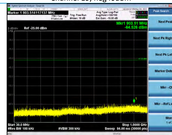
Conducted TX Spurious 30-1000 MHz Channel 25, neg40dBm
