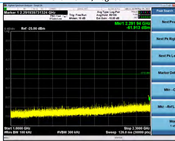
Conducted TX Spurious 1-2.3 GHz Channel 19, neg40dBm
