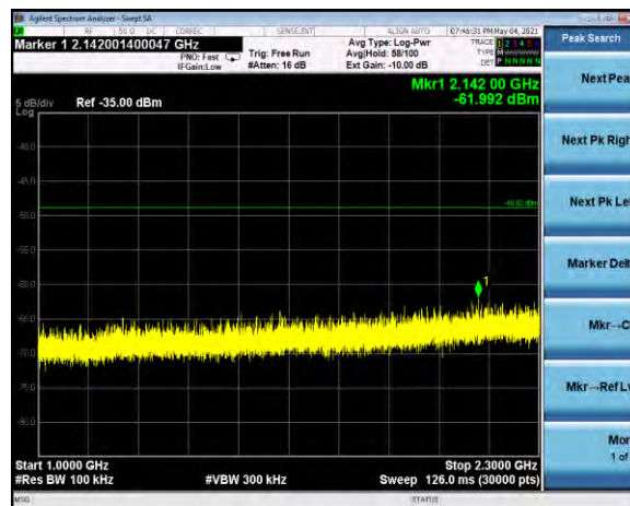
Conducted TX Spurious 1-2.3 GHz Channel 11, neg40dBm
