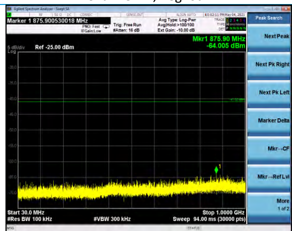
Conducted TX Spurious 30-1000 MHz Channel 19, neg40dBm
