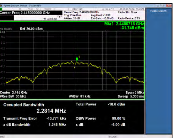
99% BW, Channel 19, neg40dBm
