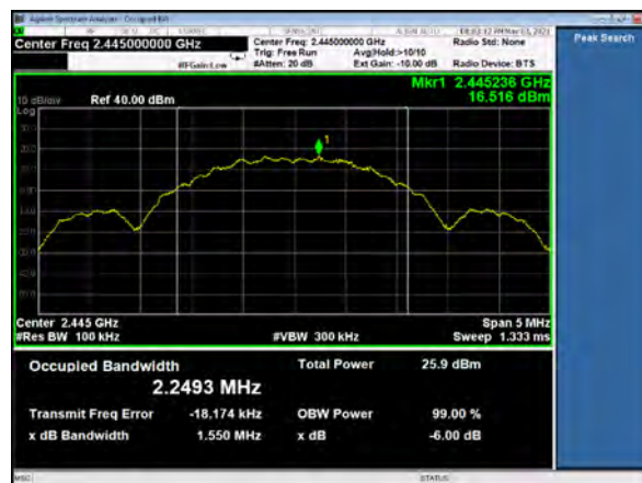
DTS BW, Channel 19, neg4dBm
