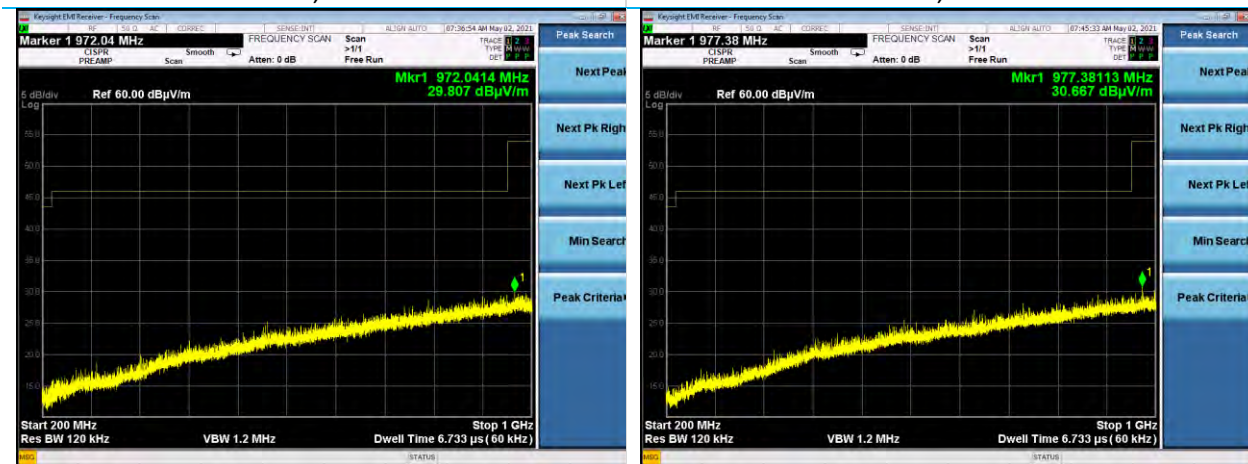
200-1000 MHz, Horizontal Antenna Vertical EUT, Channel 19
