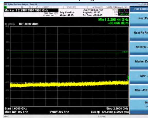
Conducted TX Spurious 1-2.3 GHz Channel 25, neg4dBm
