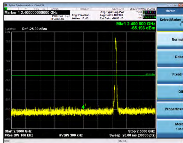
Conducted TX Spurious 2.3-2.5 GHz Channel 19, neg40dBm
