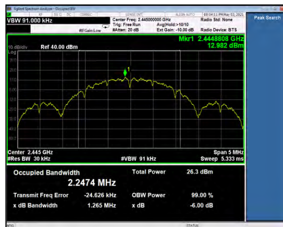
99% BW, Channel 19, neg4dBm
