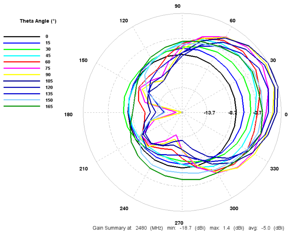
Figure 9: Total gain pattern – 2480 MHz
