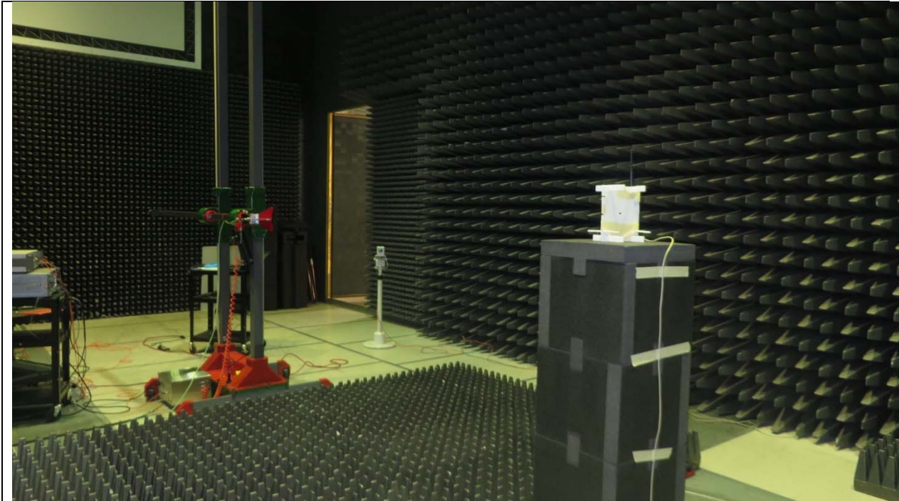
Description: TX Spurious Emissions (Radiated)
