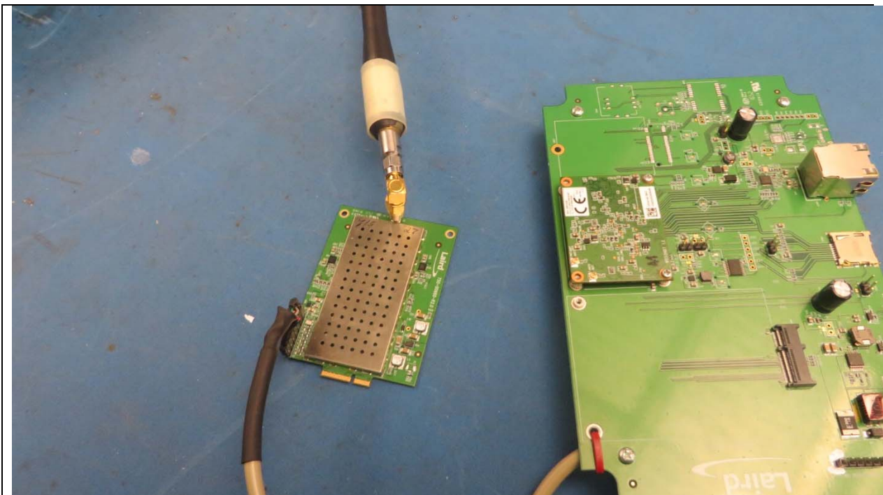
Description: Conducted RF Measurements
