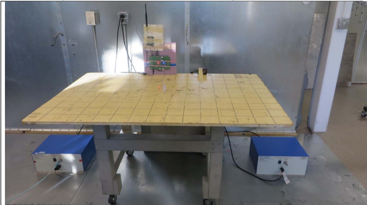
Description: AC Mains Conducted Emissions
