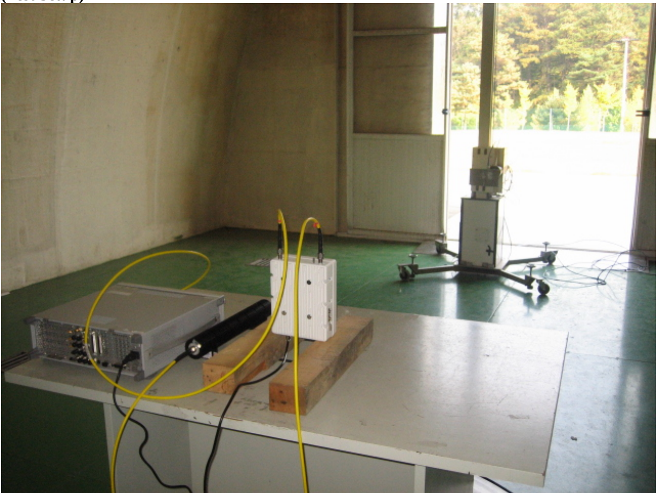
(Test Setup)
