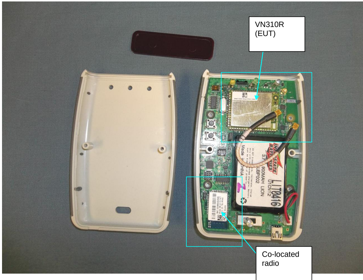
Figure 3 - Internal View
