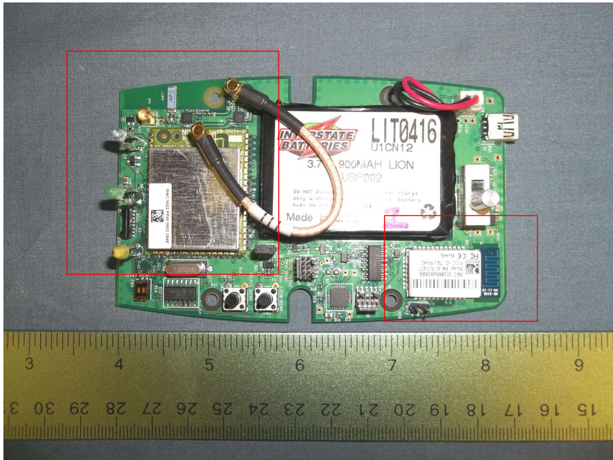
Photo 4 Host device with both radio modules
