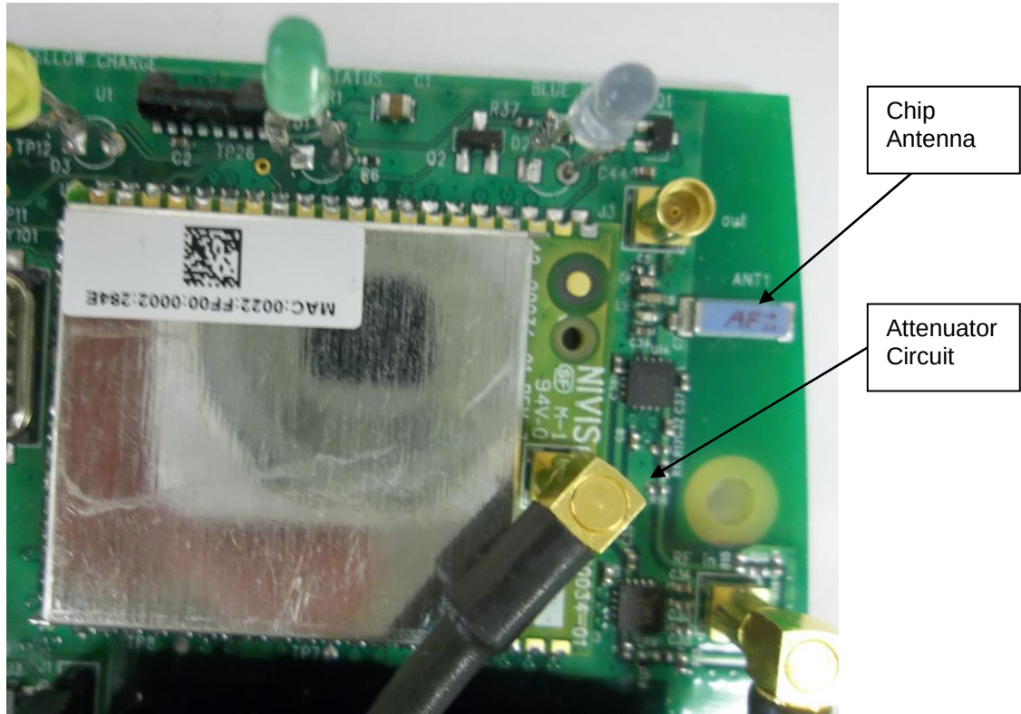
Photo 6 Top View NIVIS VN310 radio with Chip Antenna and attenuator Circuit
