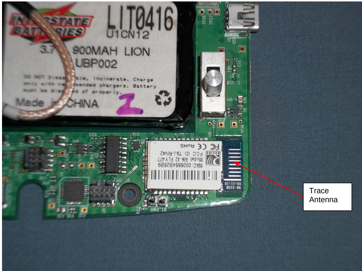
Photo 7 Co-located Radio #2
