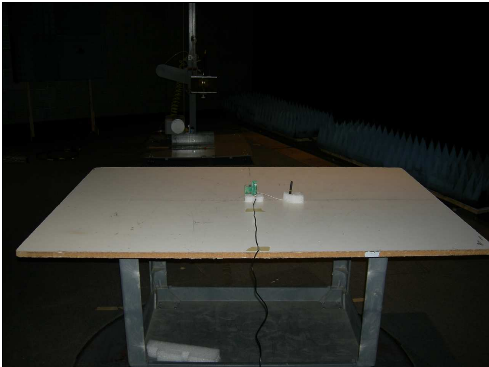
Figure 6: Radiated Emissions Test Setup – ZPOS
