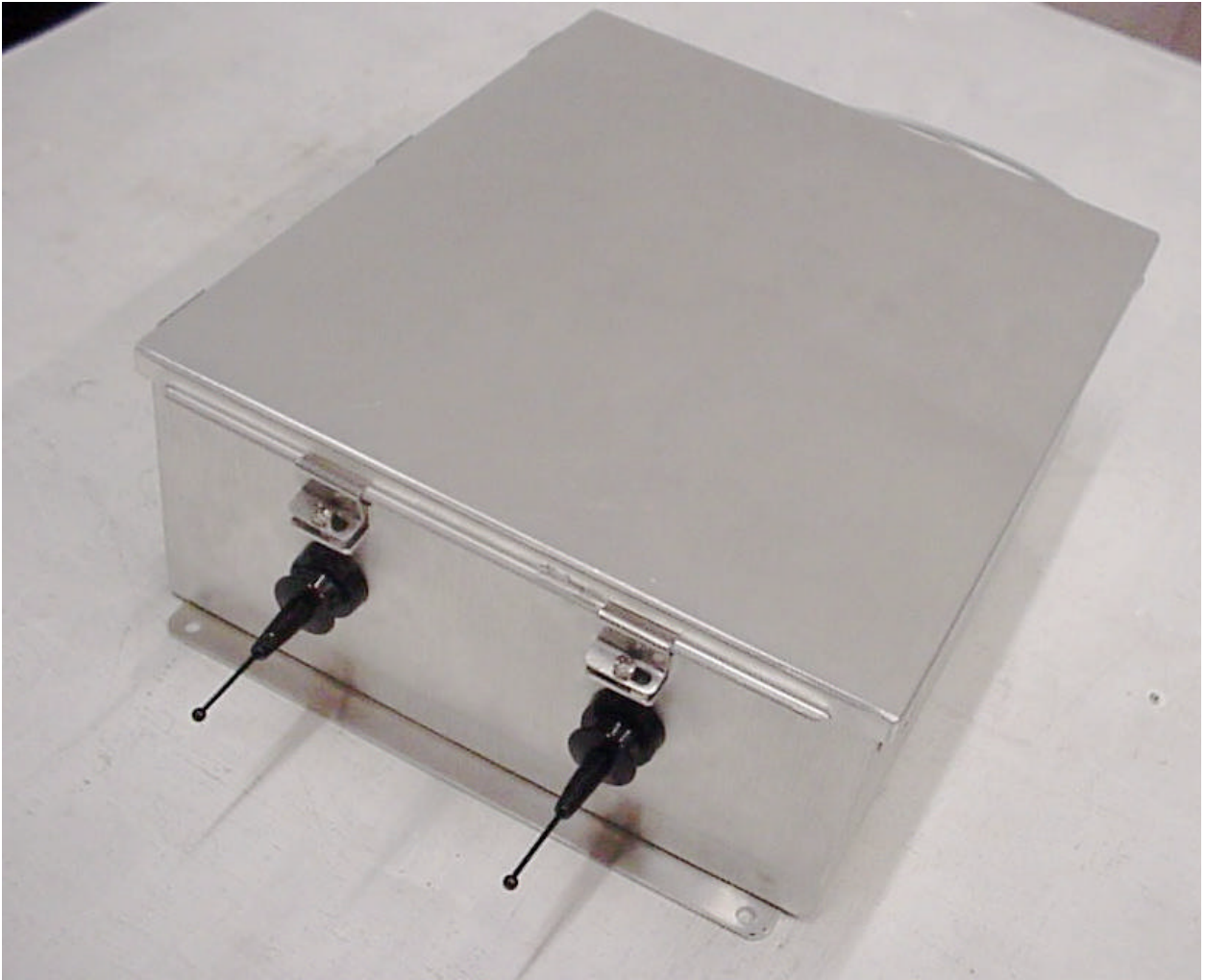
Photo 1. View Housing / Test Jig Showing Stub Antennas
