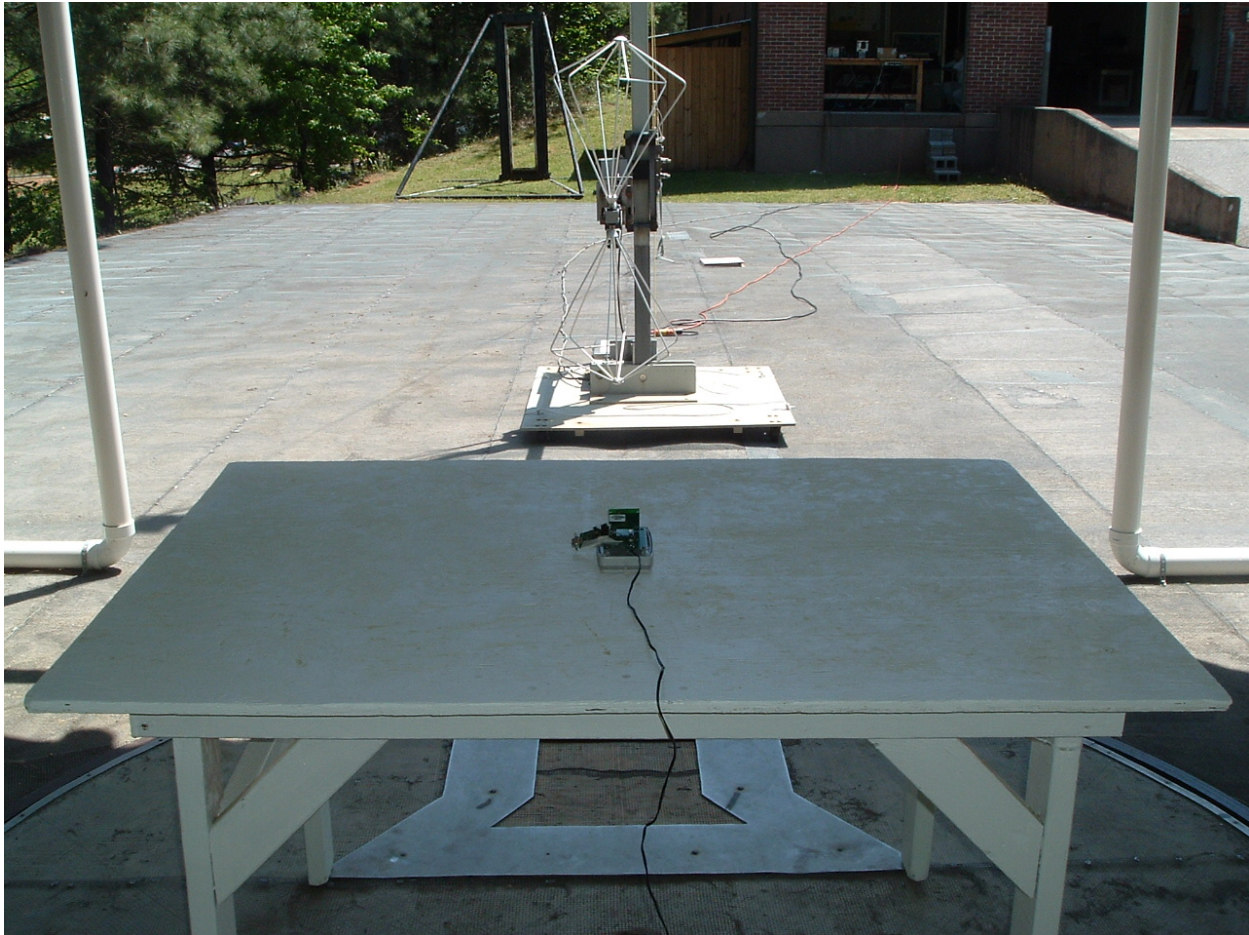
Figure 5 - Digital Radiated Emissions Measurement Setup (Rear View)
