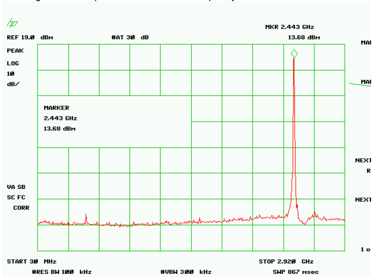
Figure 6- Antenna Conducted Spurious Emissions – CFR 15.247 (d) - Mid Channel, Part 1
