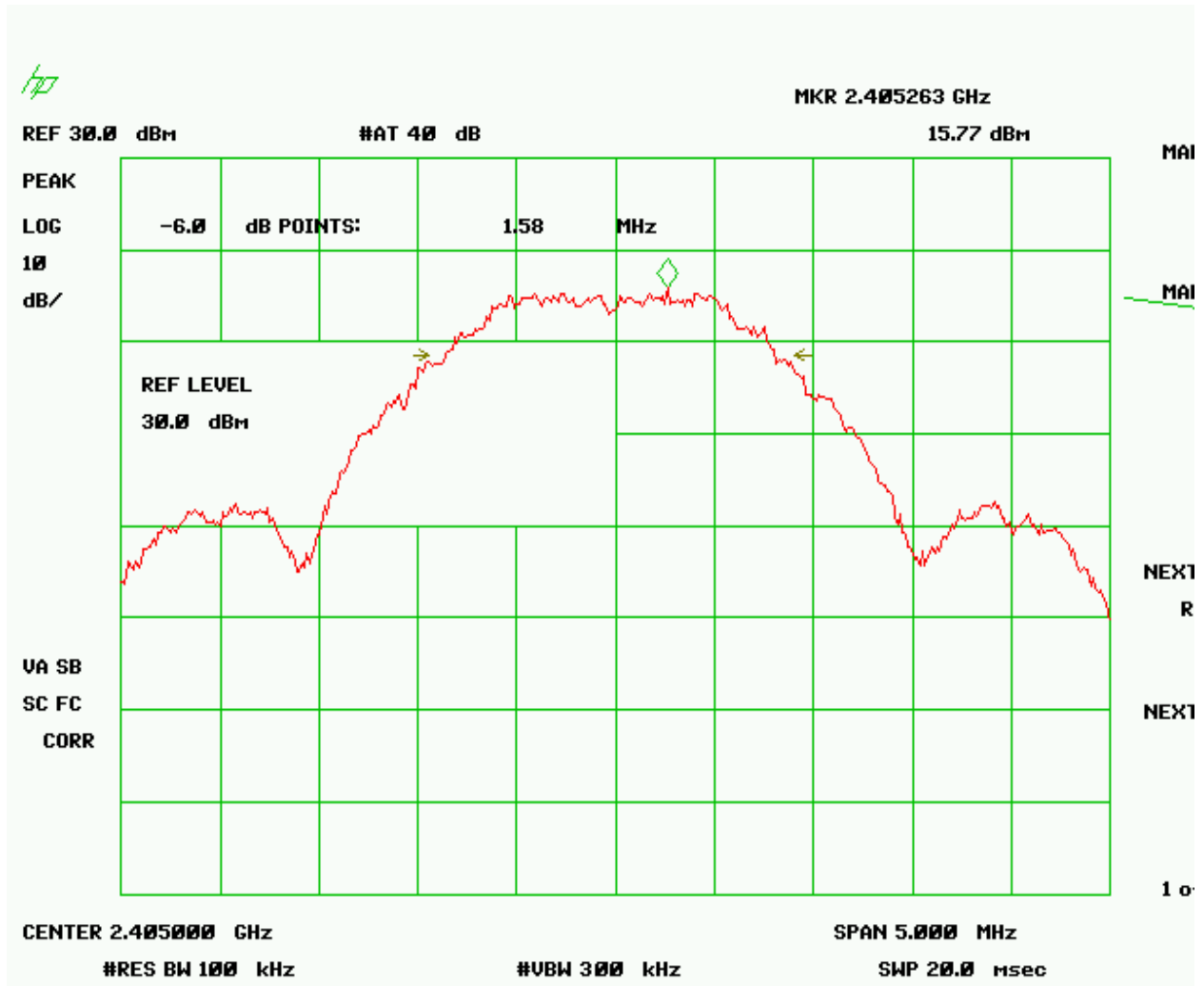
Figure 16 - Six (6) dB Bandwidth - 15.247 (a)(2) - Low Channel
