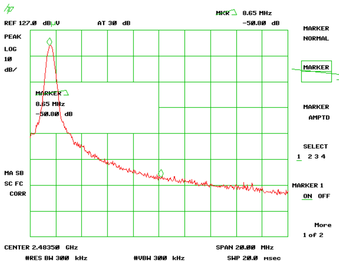
Figure 24 - Radiated Band Edge Compliance – High Channel-Peak (Tested with Antenna 1)
