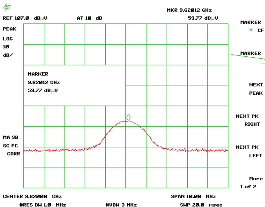
Figure 15 - Peak Radiated Spurious Emission 15.247(d) Antenna 1 Worse-case High Channel 3 rd Harmonic
