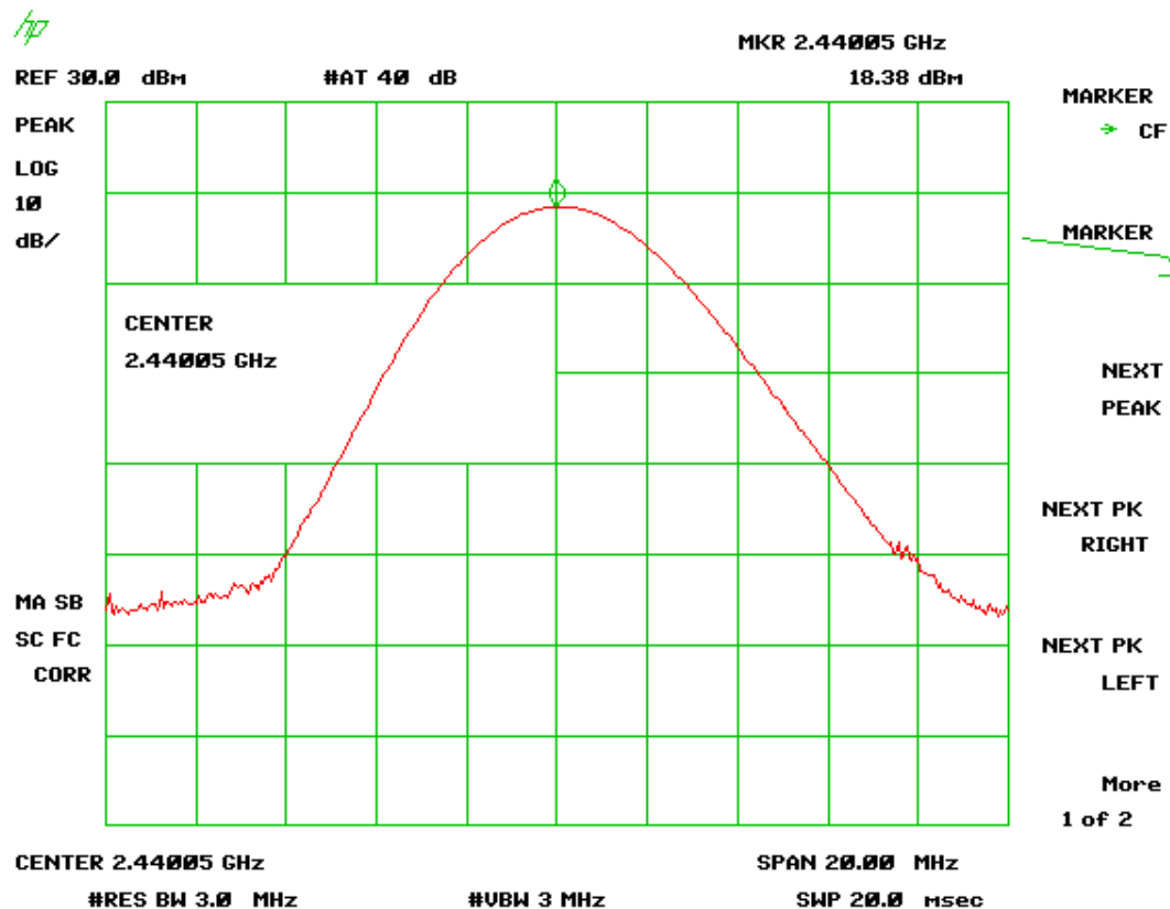
Figure 20 - Peak Antenna Conducted Output Power, Mid Channel
