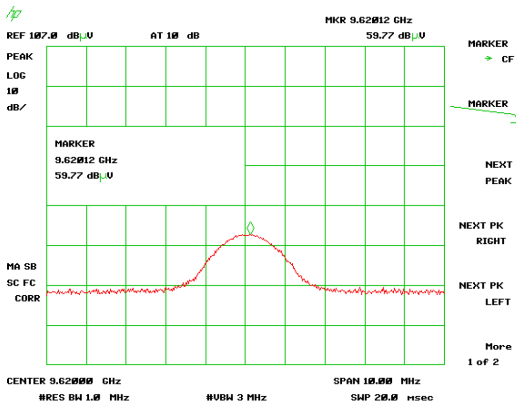
Figure 11 - Peak Radiated Spurious Emission 15.247(d) Antenna 1 Worse-case Low Channel 3 rd Harmonic
