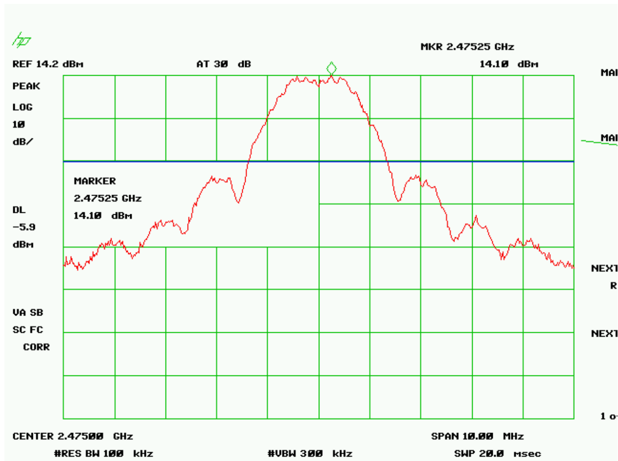
Figure 23 - Conducted Band Edge Compliance – High Channel-Peak
