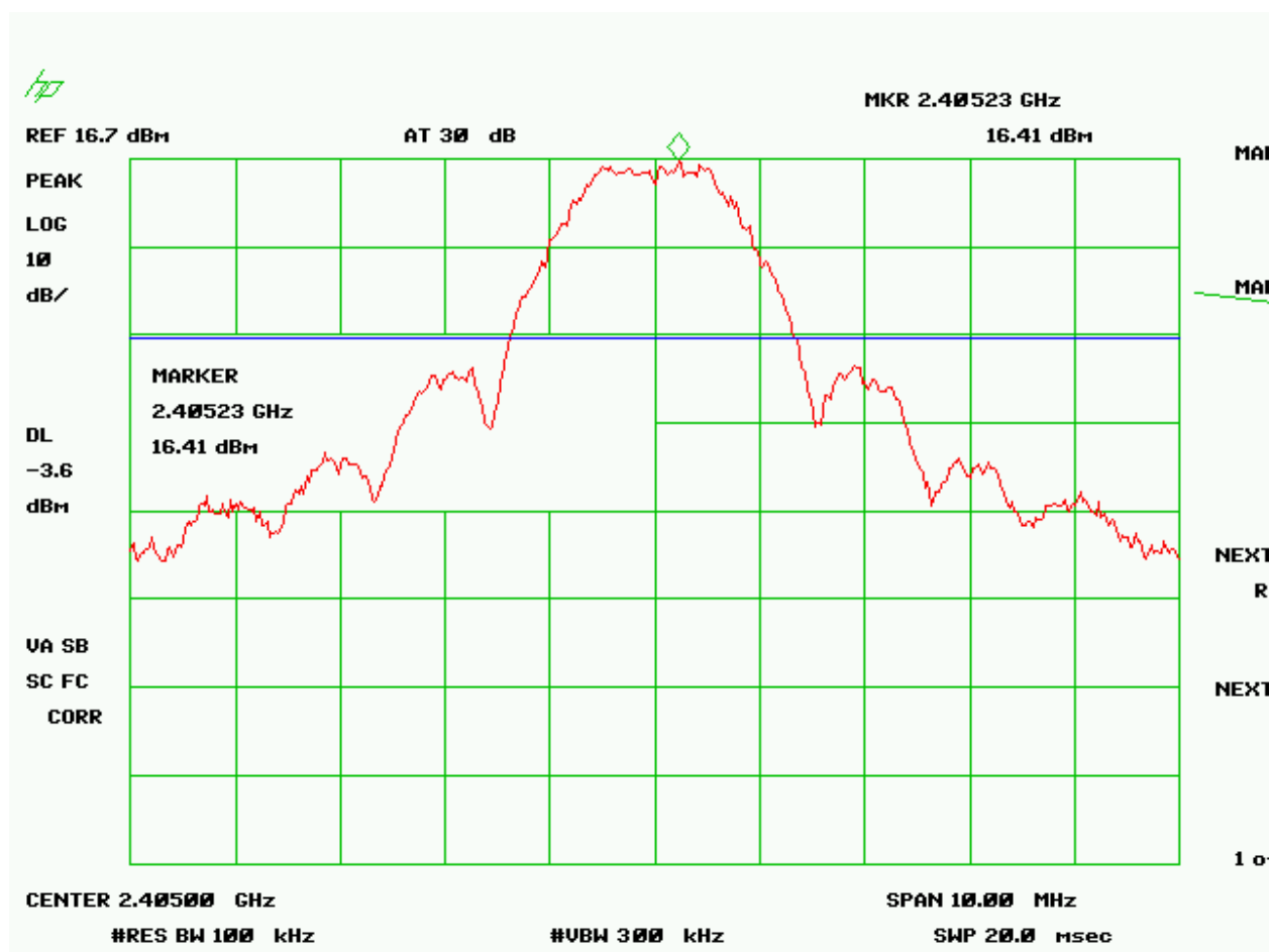
Figure 22 - Conducted Band Edge Compliance – Low Channel-Peak
