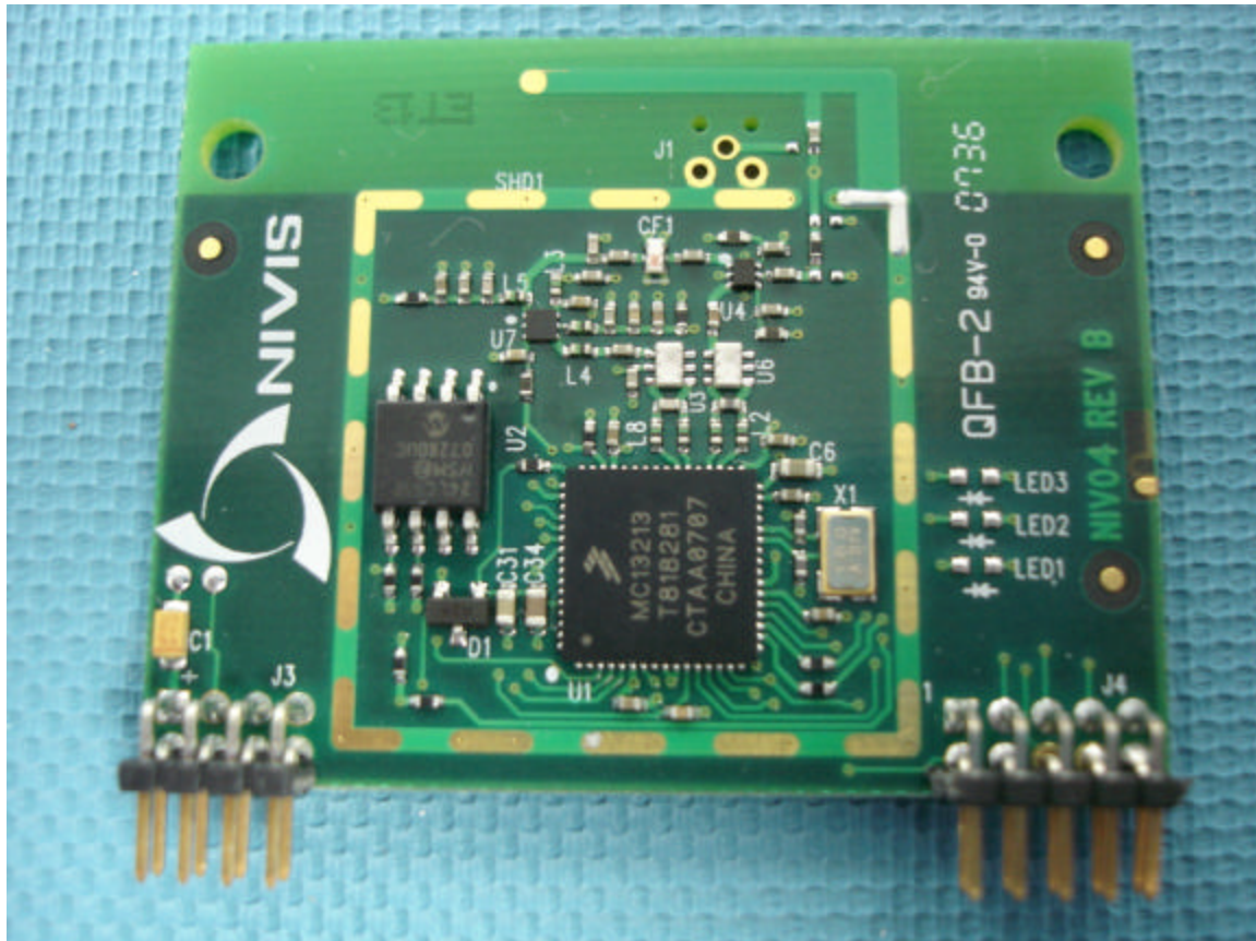
Front View of Nivis Module Board, without Shield
