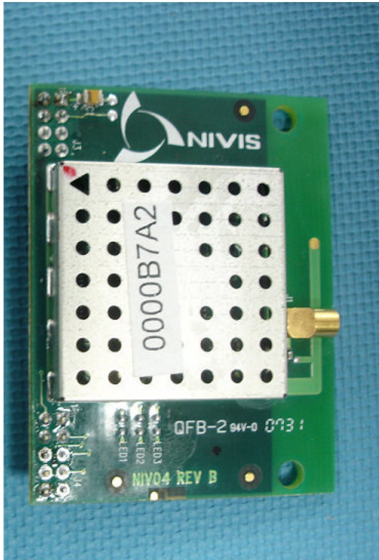
Front View of Nivis Module Board, with Shield
