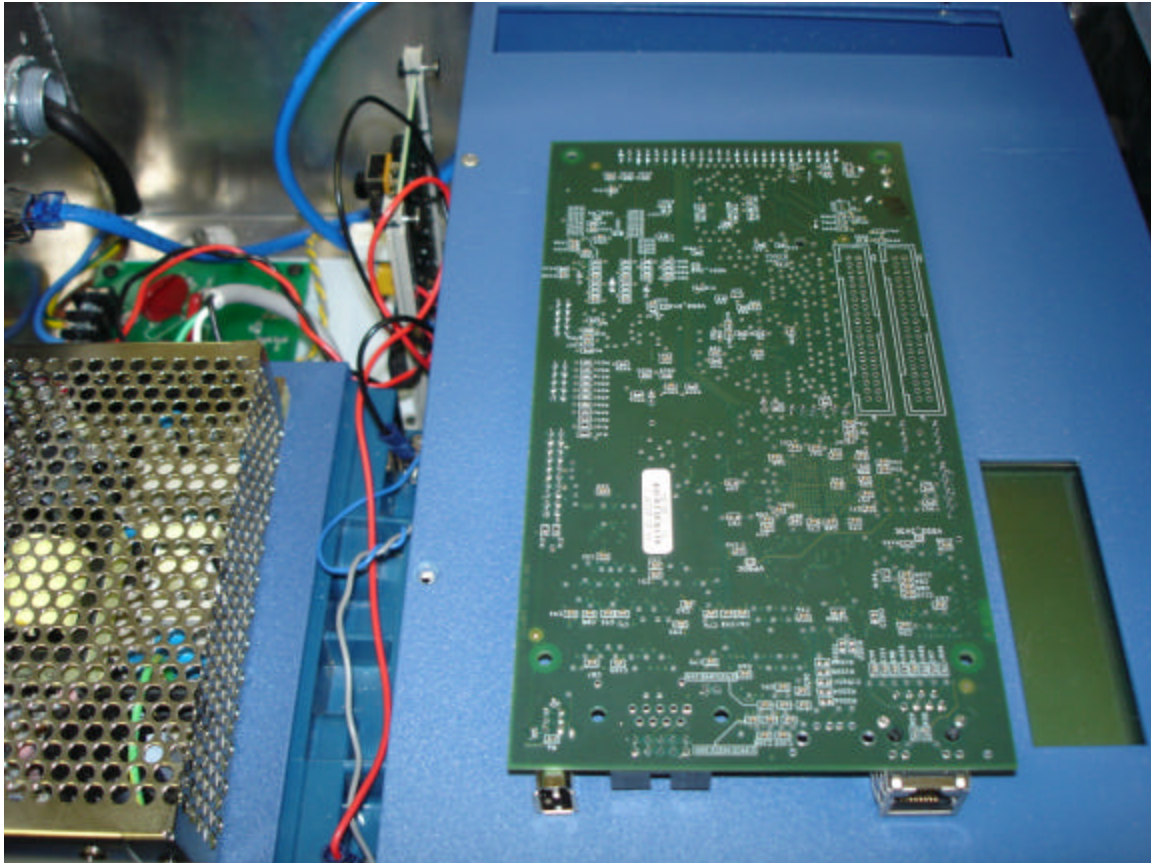
Back View of Internal Boards
