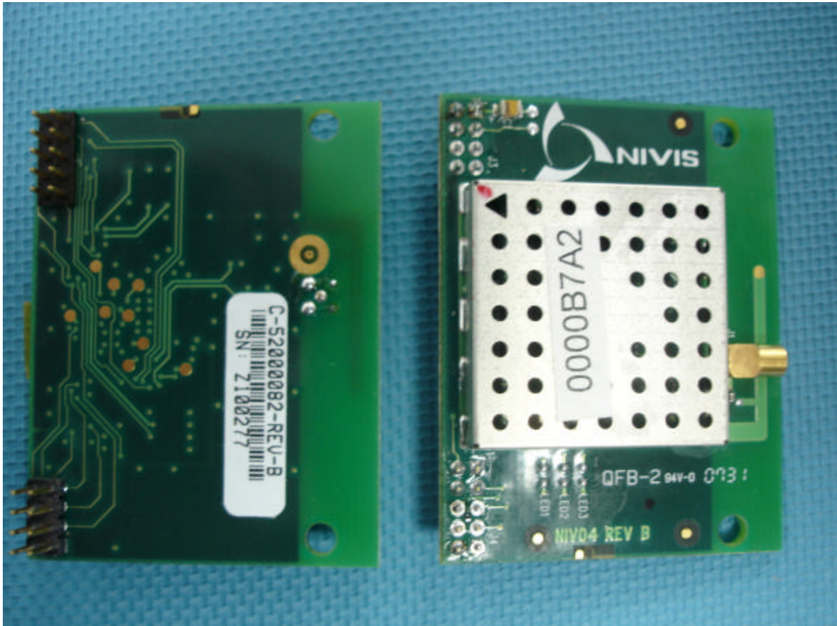
Figure 34. Photograph Top and Bottom of 2.4 GHz module
