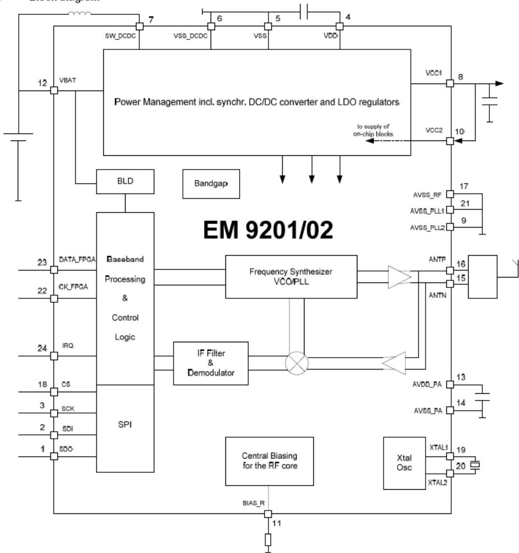
1.1 Block diagram
