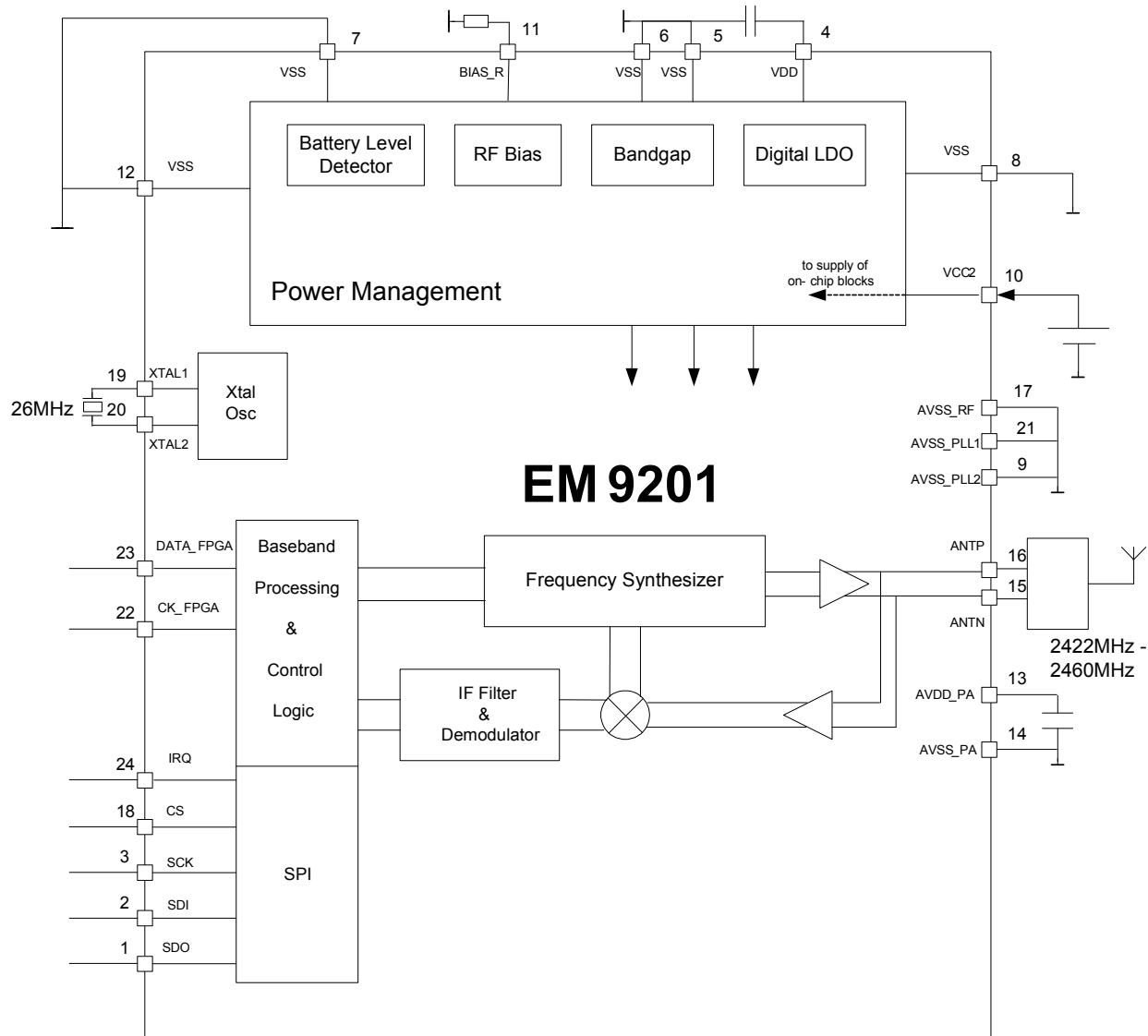
Figure 1.1: Simplified block diagram. Not all external components shown
