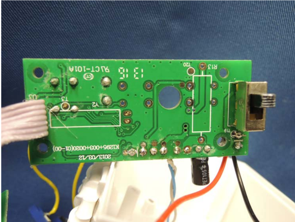
Disney Continuity Daisy Main PCB solder side
