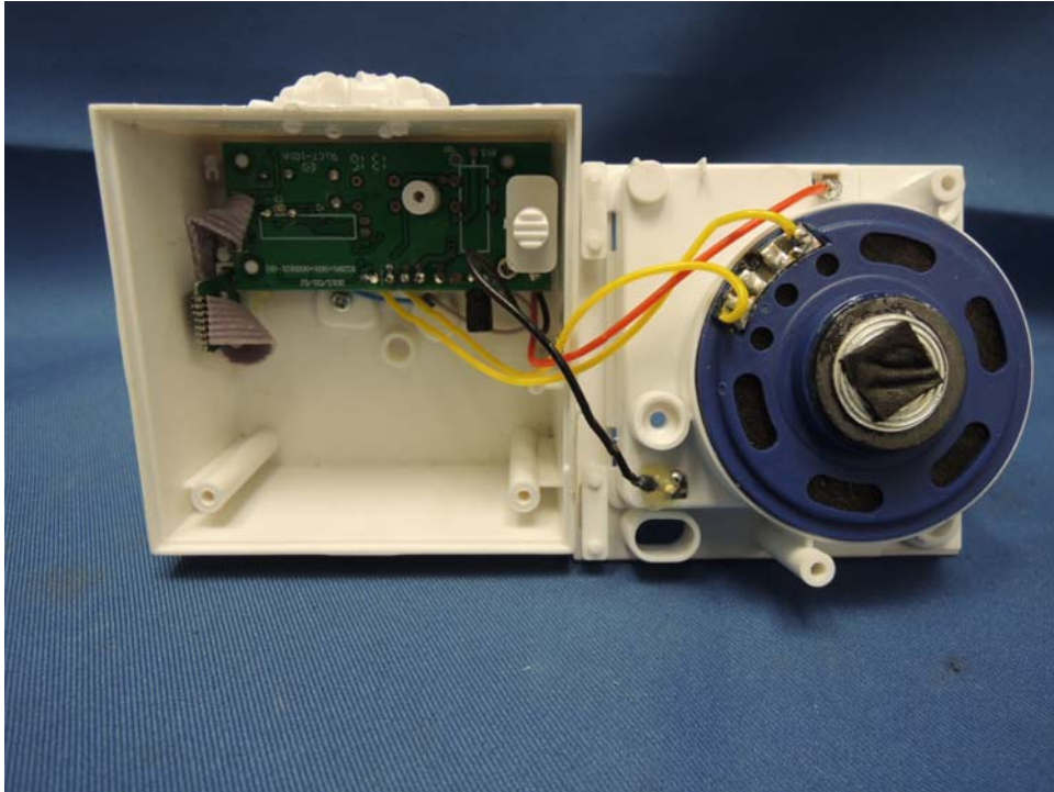
Disney Continuity Daisy assembly
