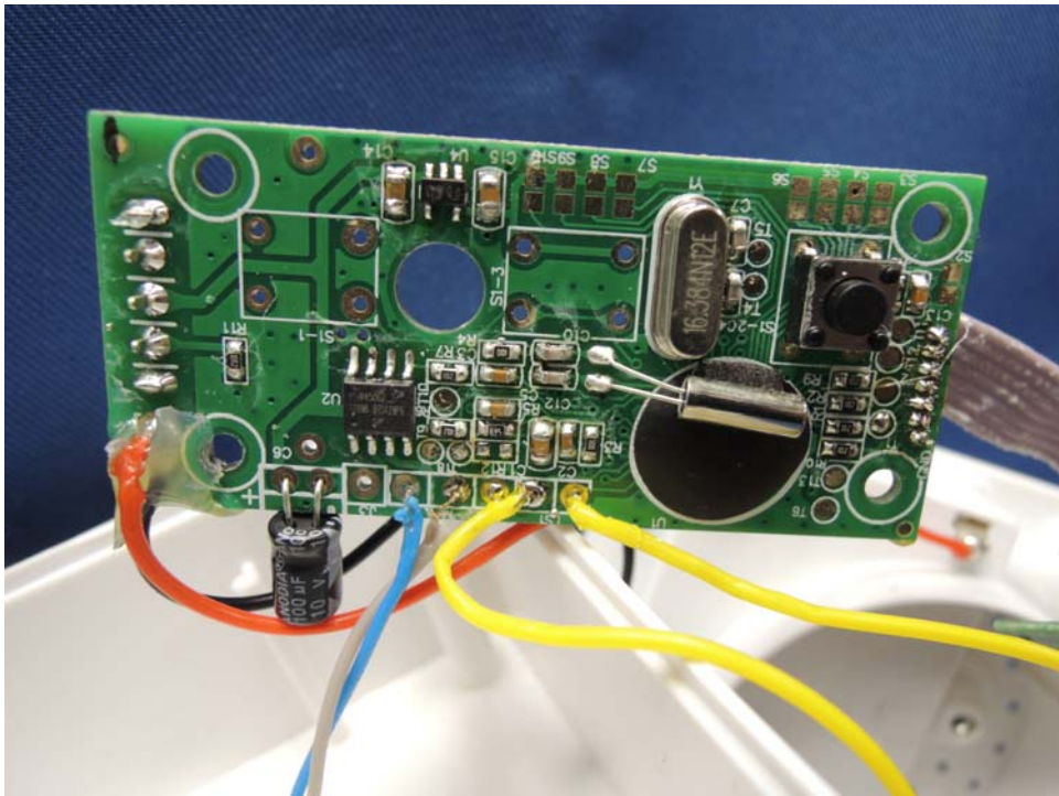
Disney Continuity Daisy Main PCB comp side
