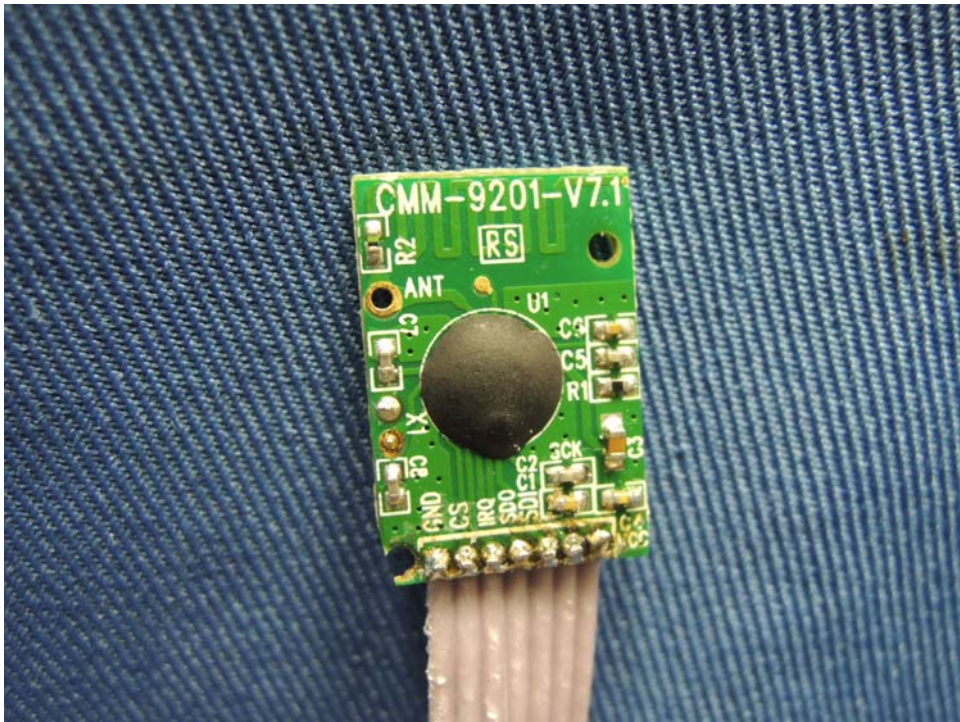
Disney Continuity Daisy RF module PCB front side
