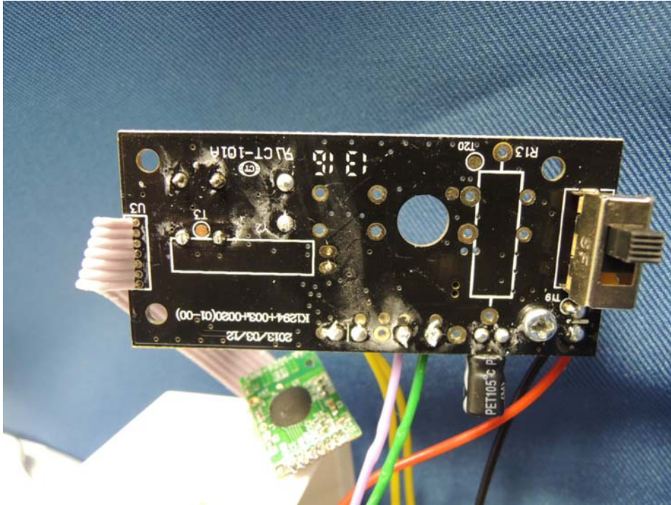
Disney Continuity Goofy Main PCB solder side
