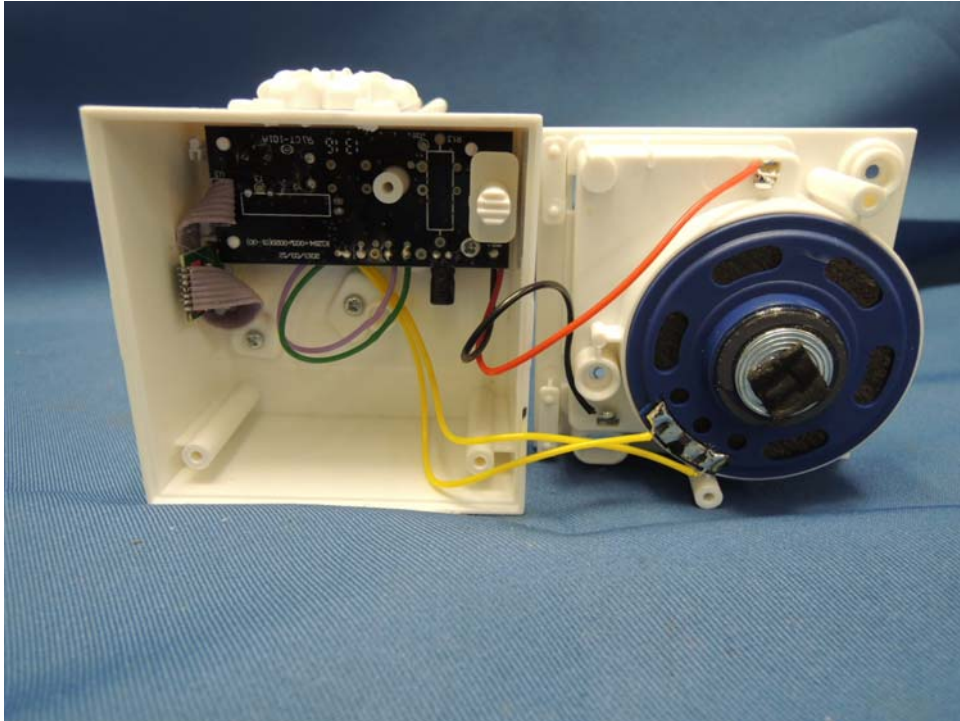
Disney Continuity Goofy assembly
