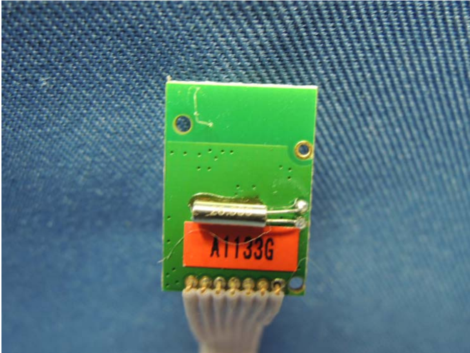
Disney Continuity Goofy RF module PCB rear side (View 1)
