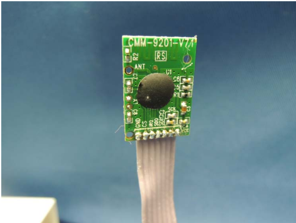
Disney Continuity Goofy RF module PCB front side
