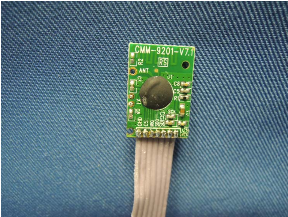
Disney Continuity Donald RF module PCB front side
