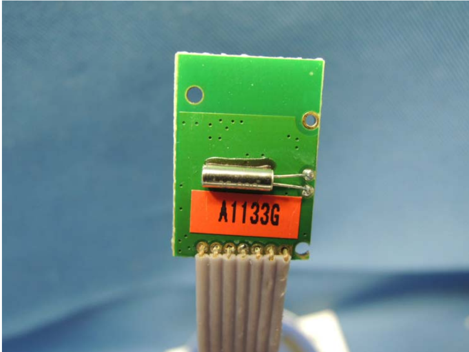
Disney Continuity Donald RF module PCB rear side (View 1)
