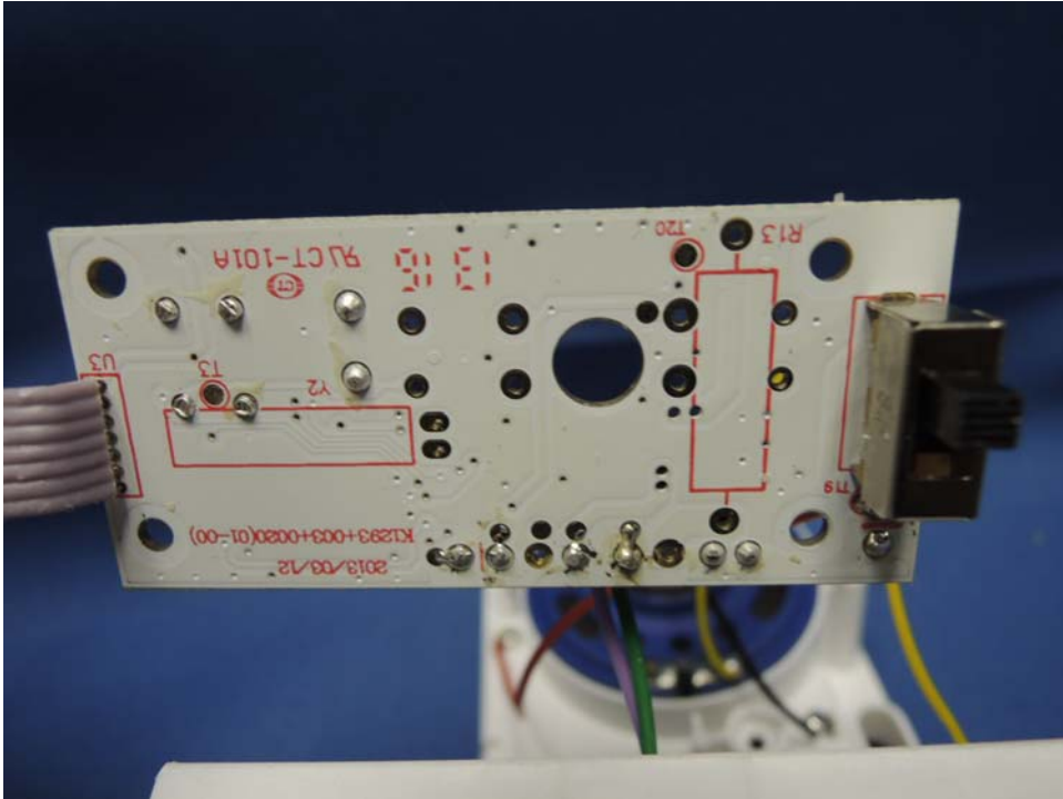
Disney Continuity Donald Main PCB solder side
