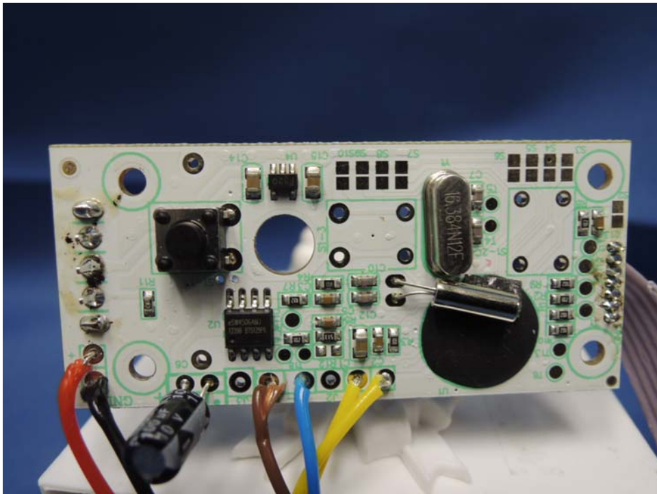
Disney Continuity Mickey Main PCB comp side
