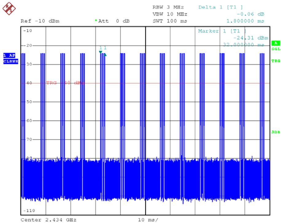
Timing Plot – Pursuant to FCC Part 15 Section 15. 249 Requirement
