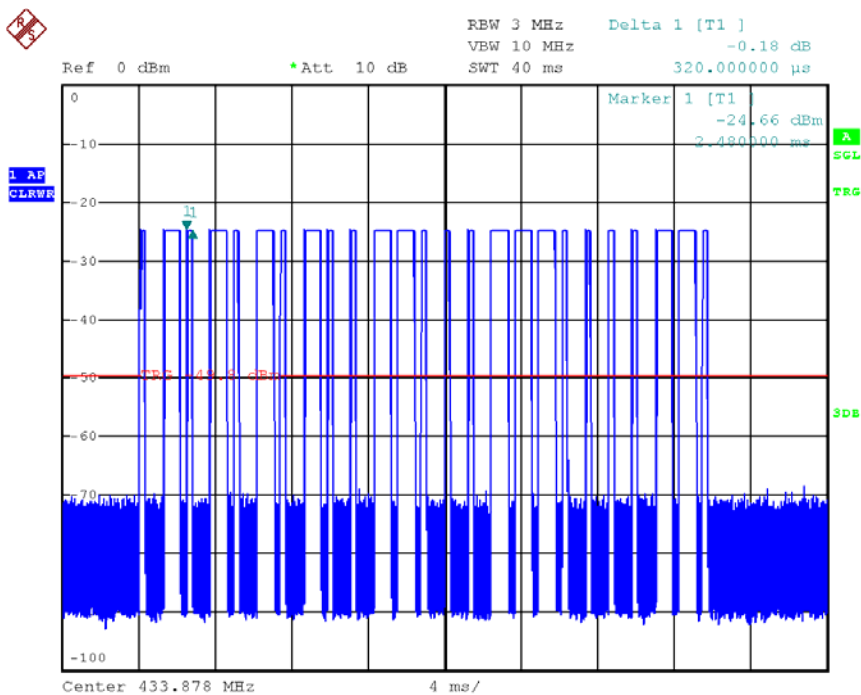
Timing Plot – Pursuant to FCC Part 15 Section 15.231(a)
