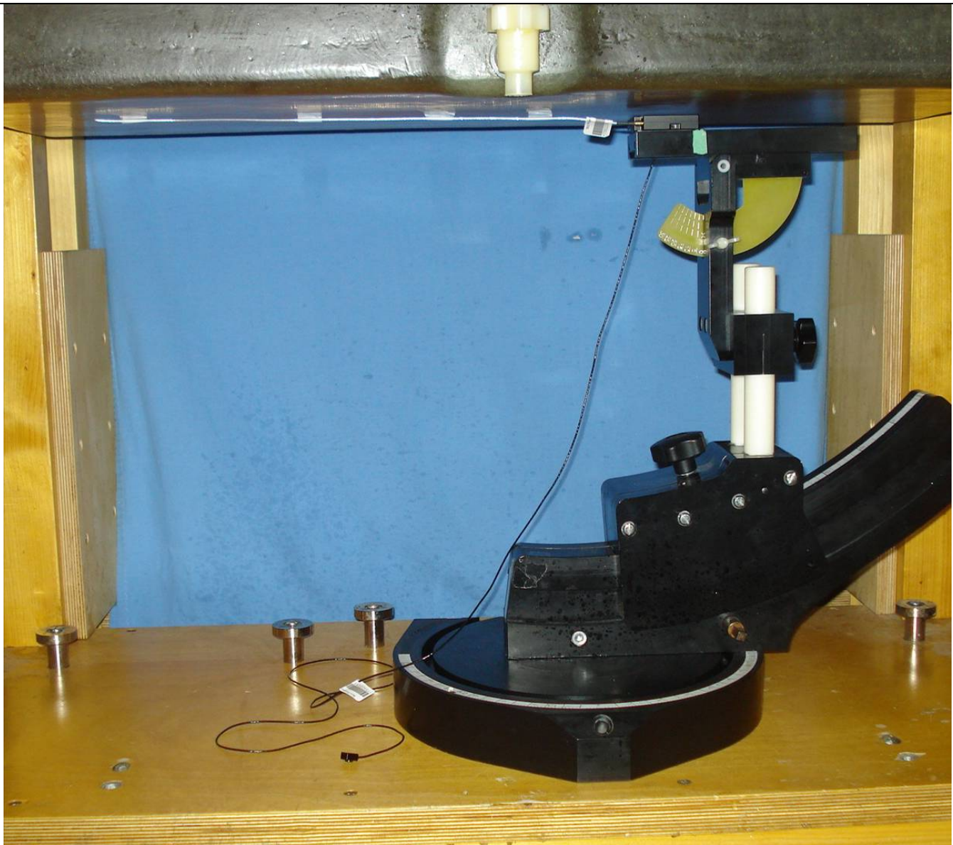
Body-Worn Test Setup
