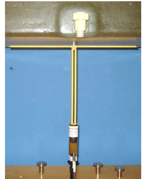
SPEAG 300 MHz Validation Dipole Setup
