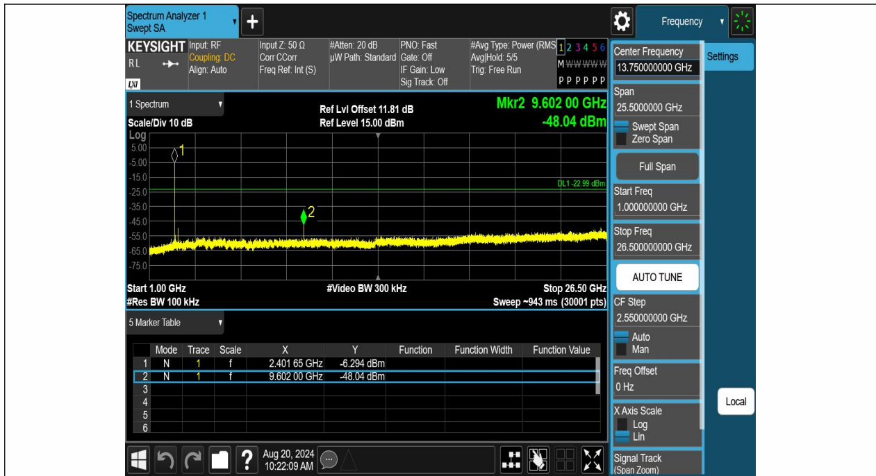
BLE_1M-Ant1-2402-1000~26500-PASS
