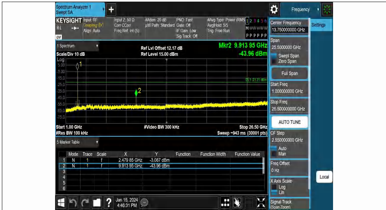
BLE_1M-Ant1-2480-1000~26500-PASS
