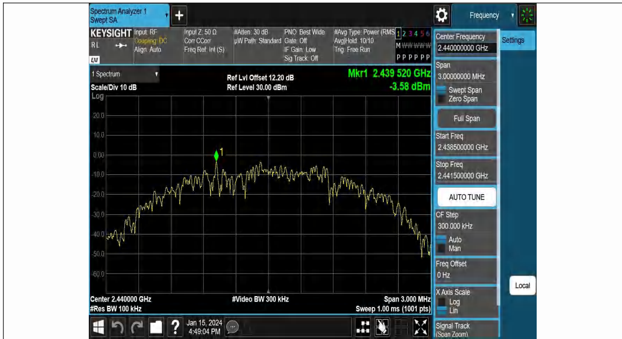
BLE_2M-Ant1-2440-0~Reference-PASS
