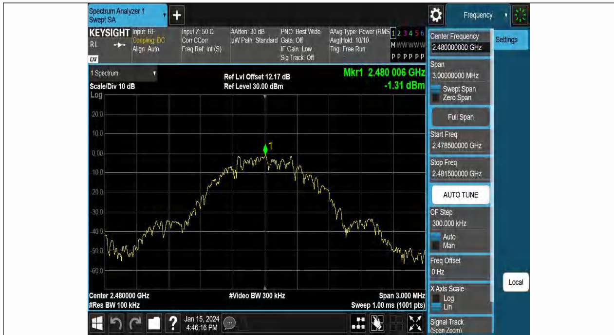
BLE_1M-Ant1-2480-0~Reference-PASS
