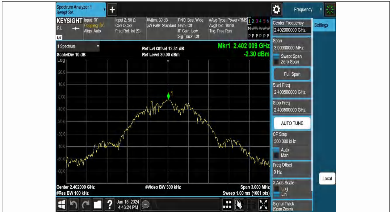
BLE_1M-Ant1-2402-0~Reference-PASS
