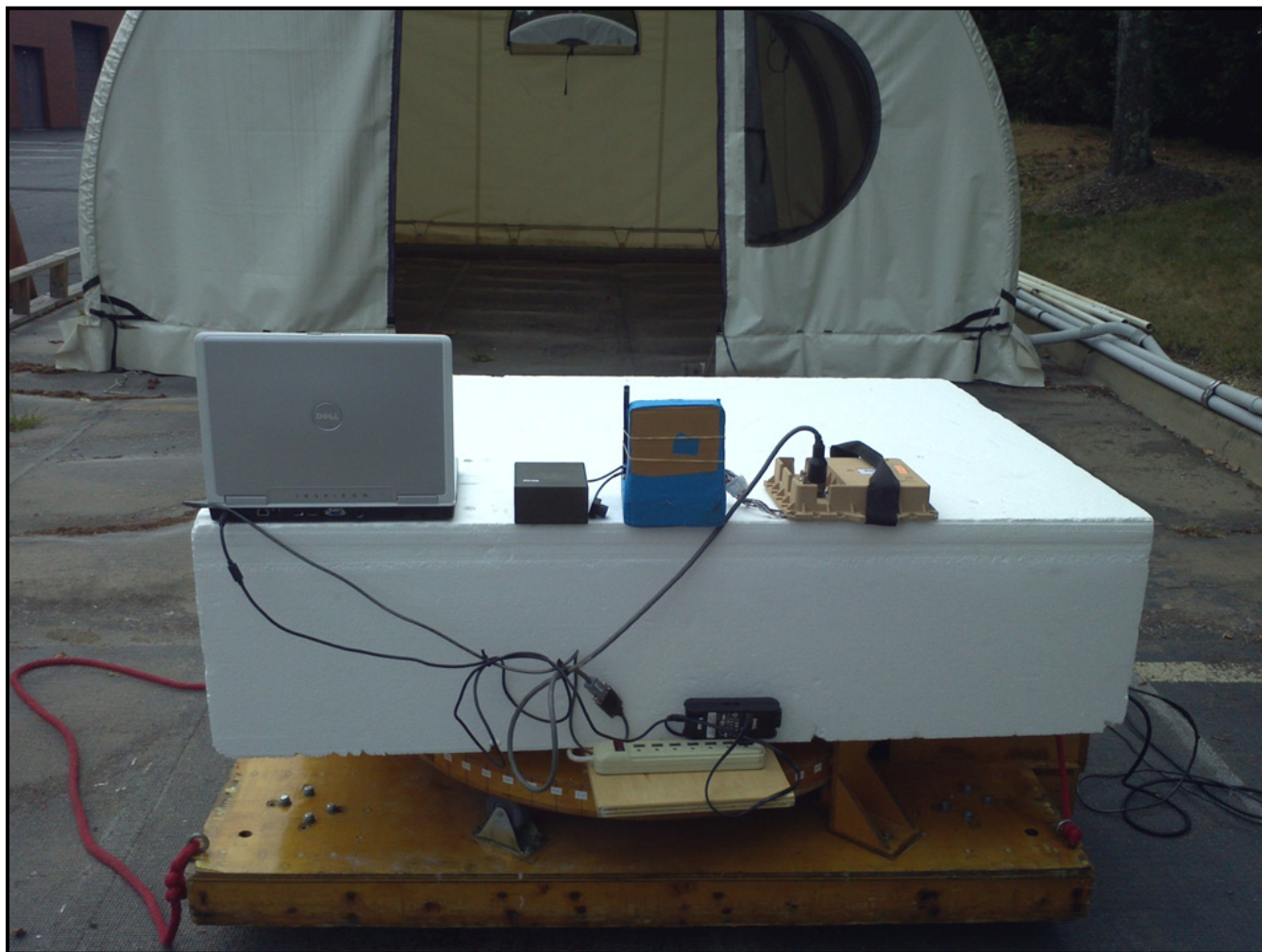
Photograph 4: Radiated Emissions – Rear View – Rubber Duck Antenna
