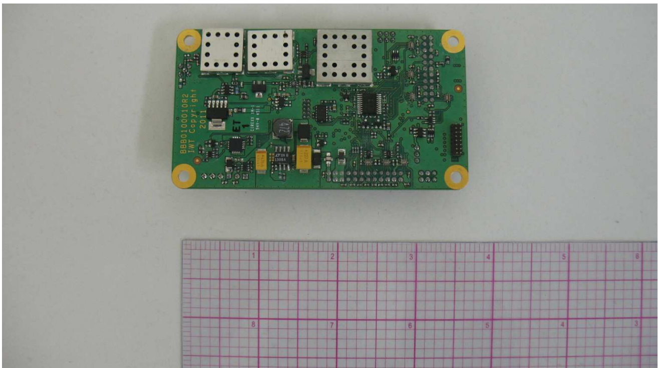
Radio PCB – Bottom View, with shields
