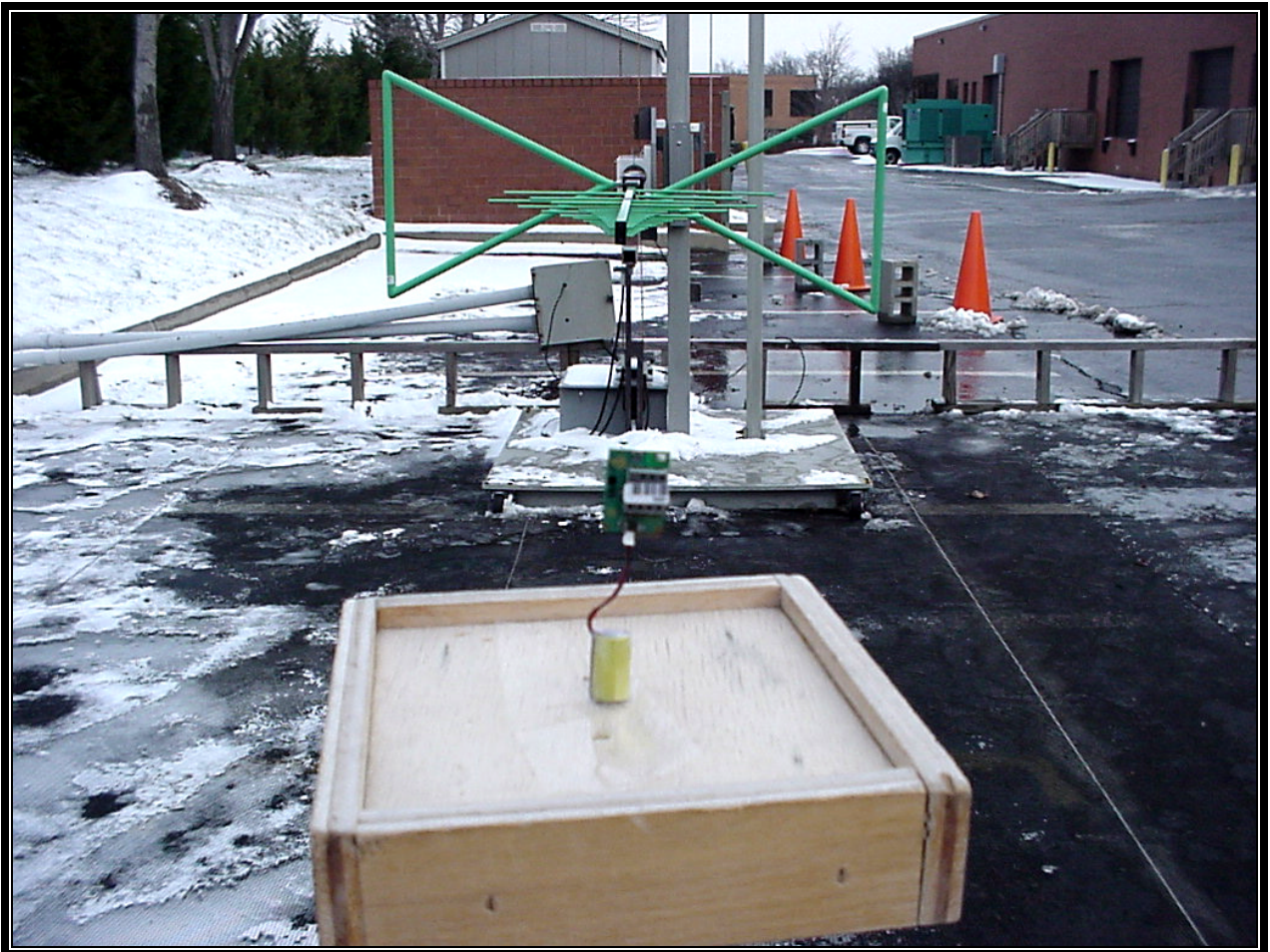
PHOTOGRAPH 1: RADIATED EMISSIONS FRONT VIEW (3 M)
