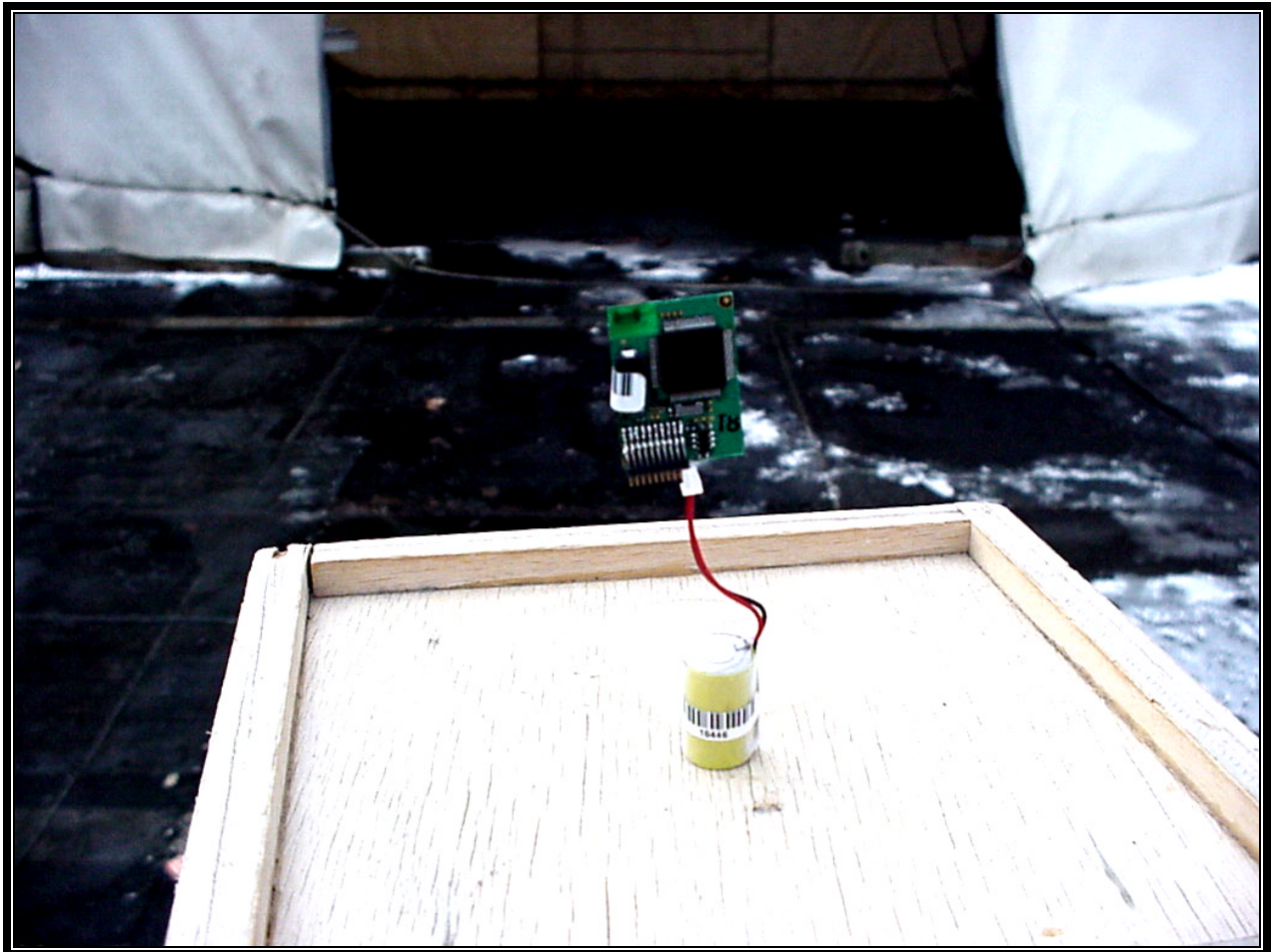
PHOTOGRAPH 2: RADIATED EMISSIONS REAR VIEW (3 M)
