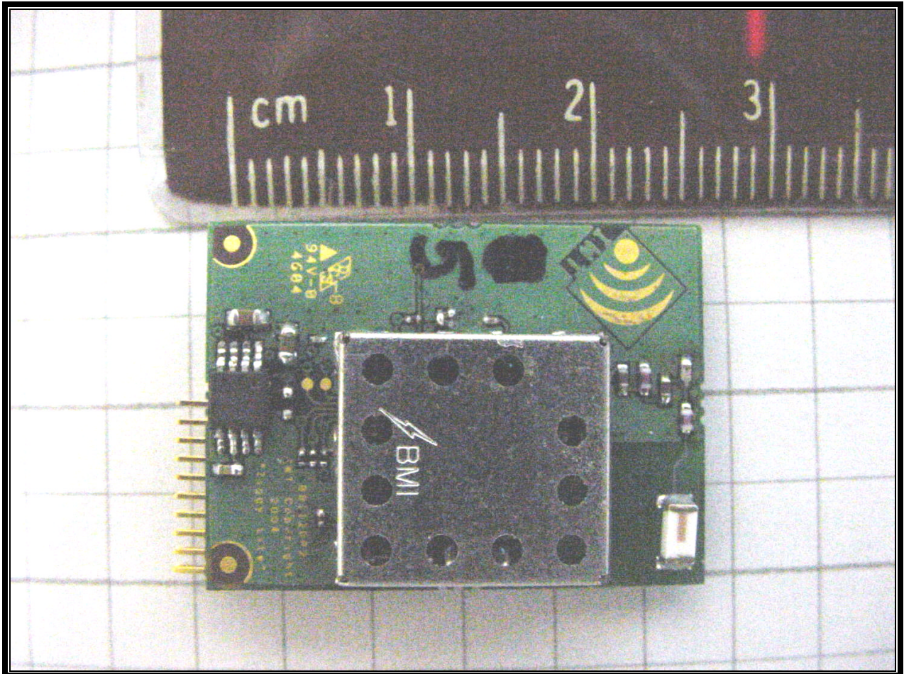
PHOTOGRAPH 6: MODULE BOTTOM VIEW WITH SHIELD
