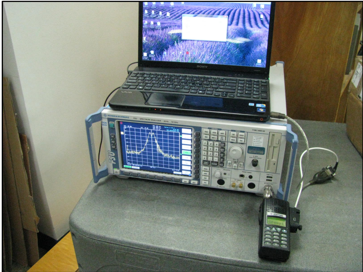
Photograph 1: Conducted Antenna Port Testing
