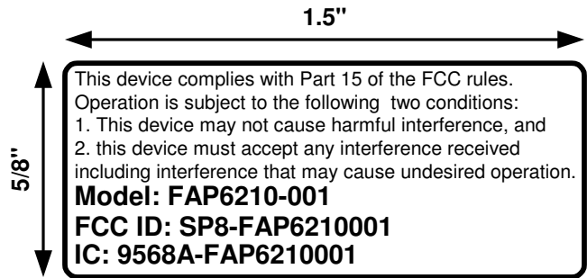
FCC Label (4X)
