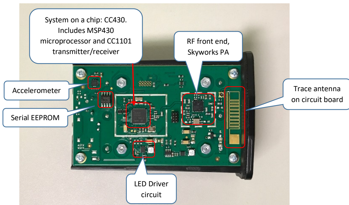
Figure 8 - Top View of Circuit Board
