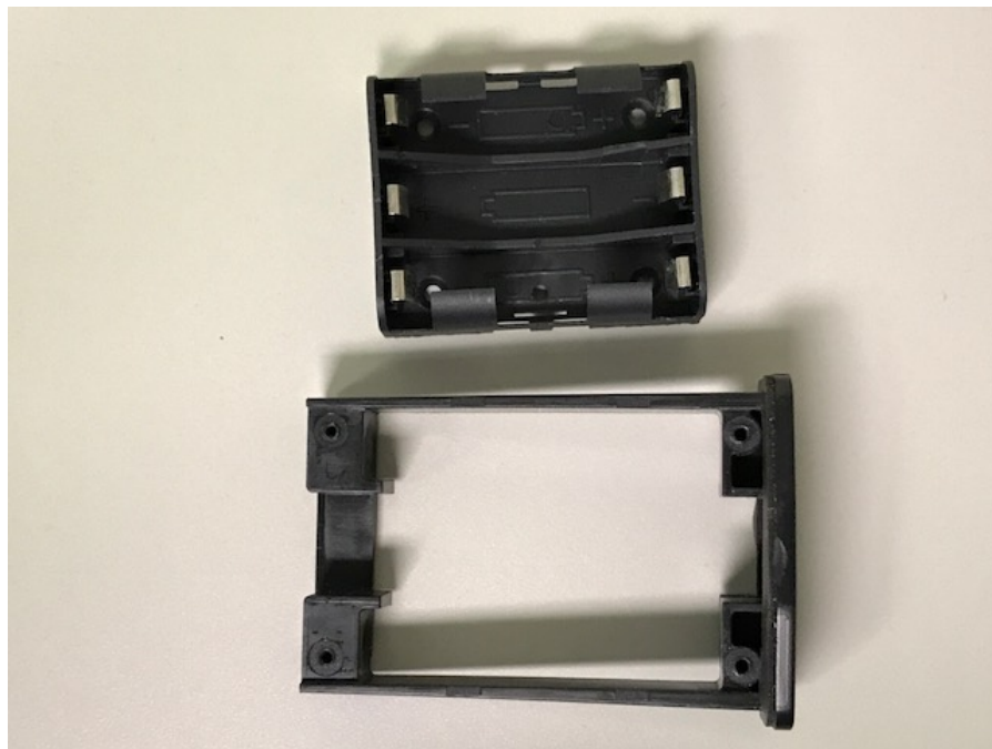
Figure 12 - Interior 'Tray' and battery holder, separated
