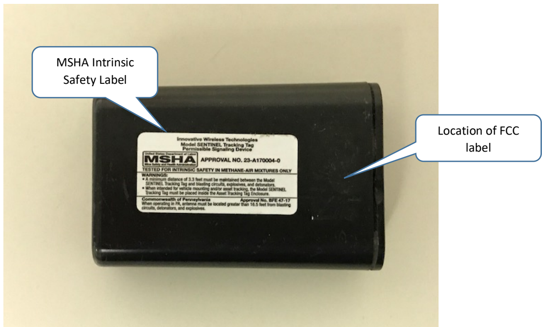
Figure 2 - Bottom view of Tracking Tag
