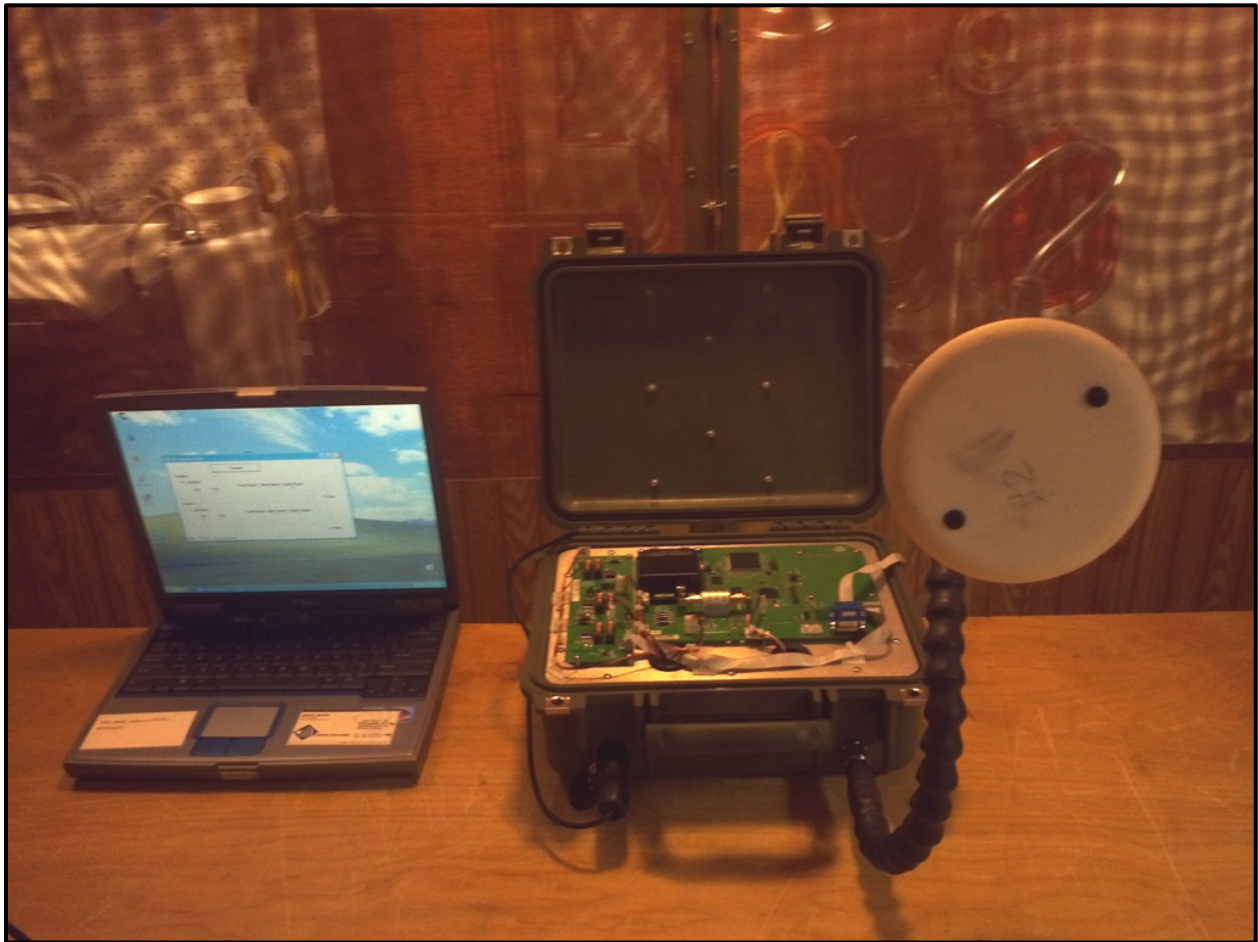
Photograph 5: Conducted AC Testing – Front View with Omni Antenna
