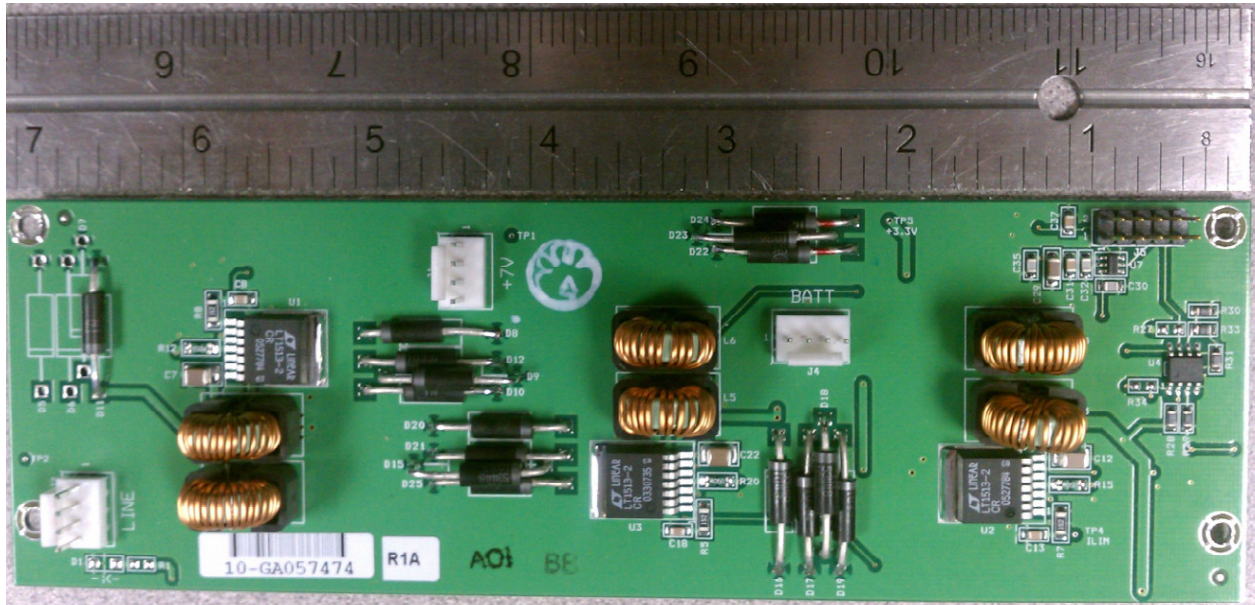
IWT PMN POWER SUPPLY BOARD TOP VIEW
