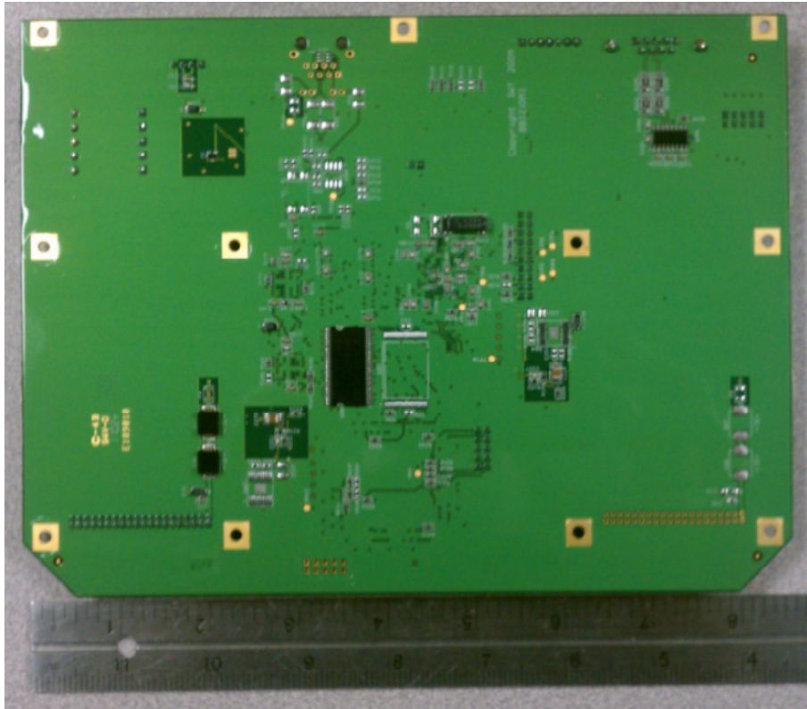
IWT PMN ROUTER BOARD BOTTOM VIEW
