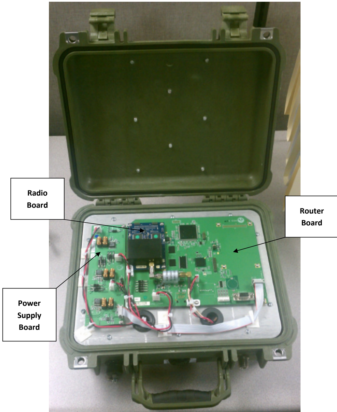
IWT PMN TOP VIEW - OPEN
