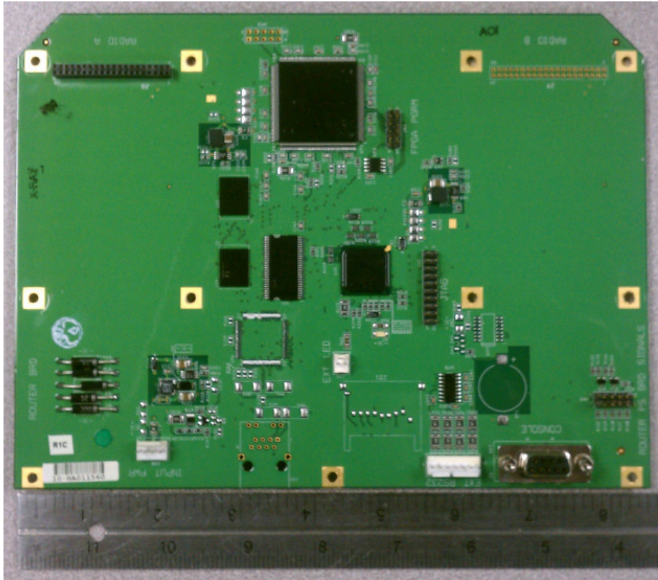
IWT PMN ROUTER BOARD TOP VIEW
