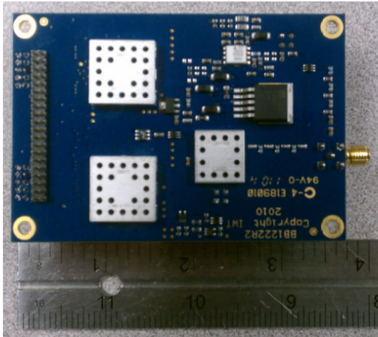
IWT PMN 900 MHz RADIO BOARD BOTTOM VIEW
