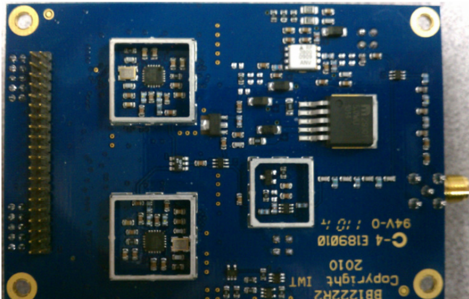
RADIO BOARD BOTTOM VIEW Close-up w/o Covers
