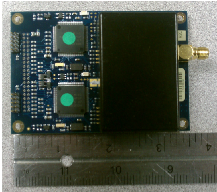
IWT PMN 900 MHz RADIO BOARD TOP VIEW
