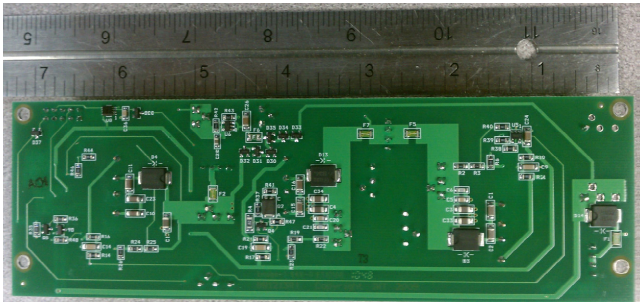
IWT PMN POWER SUPPLY BOARD BOTTOM VIEW
