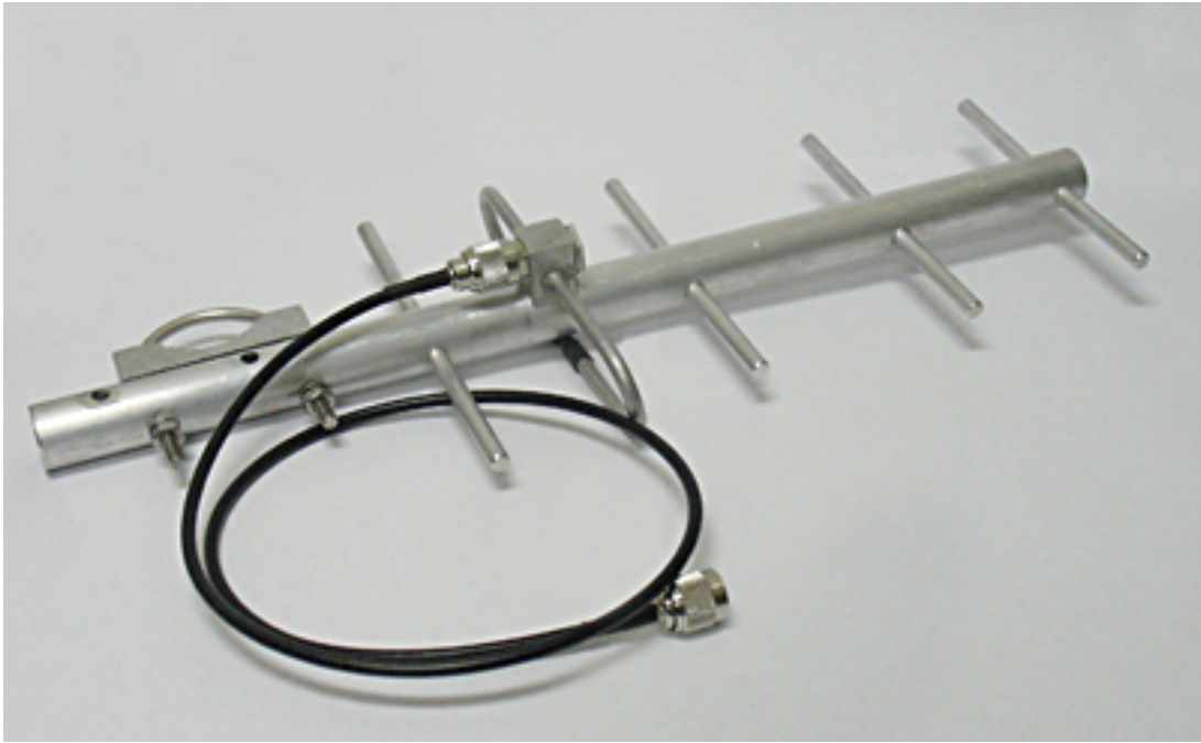
Figure 7 - Yagi direction antenna with RF cable
