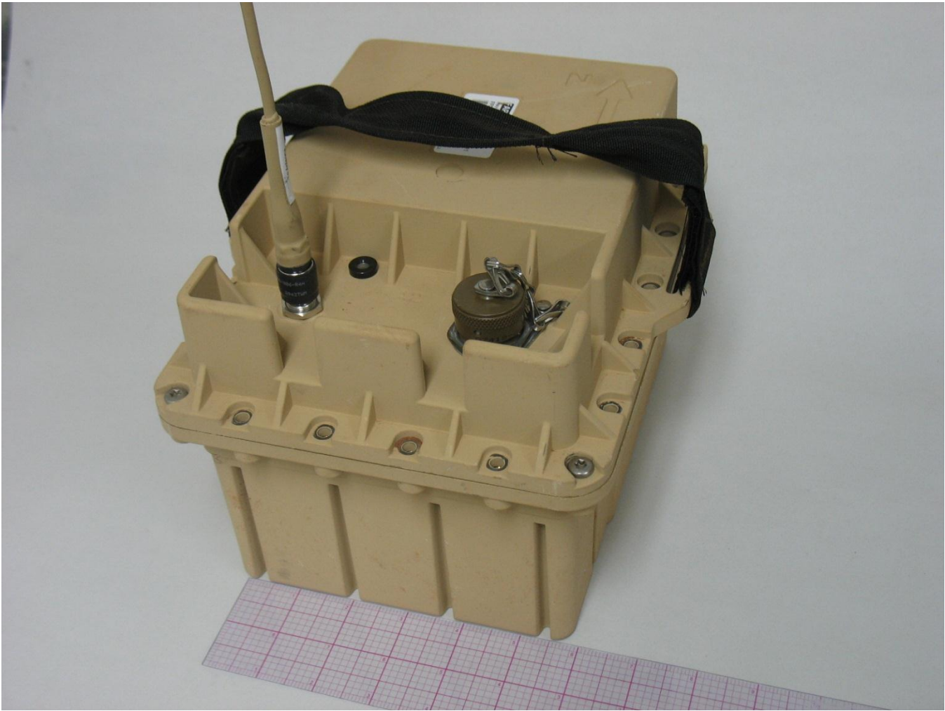
Exterior of Coyote UGS – Antenna, LED, carrying strap, and 19-pin MIL connector
