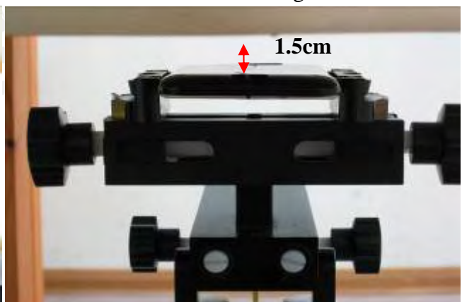
Fig.7 Body worn- EUT back to flat phantom and distance between flat phantom and mobile phone is 1.5 cm
