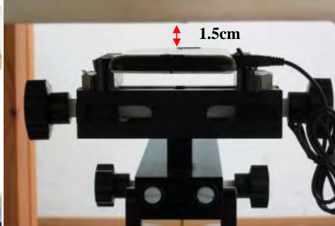
Fig.9 Body worn- EUT Front to flat phantom and distance between flat phantom and mobile phone is 1.5 cm
