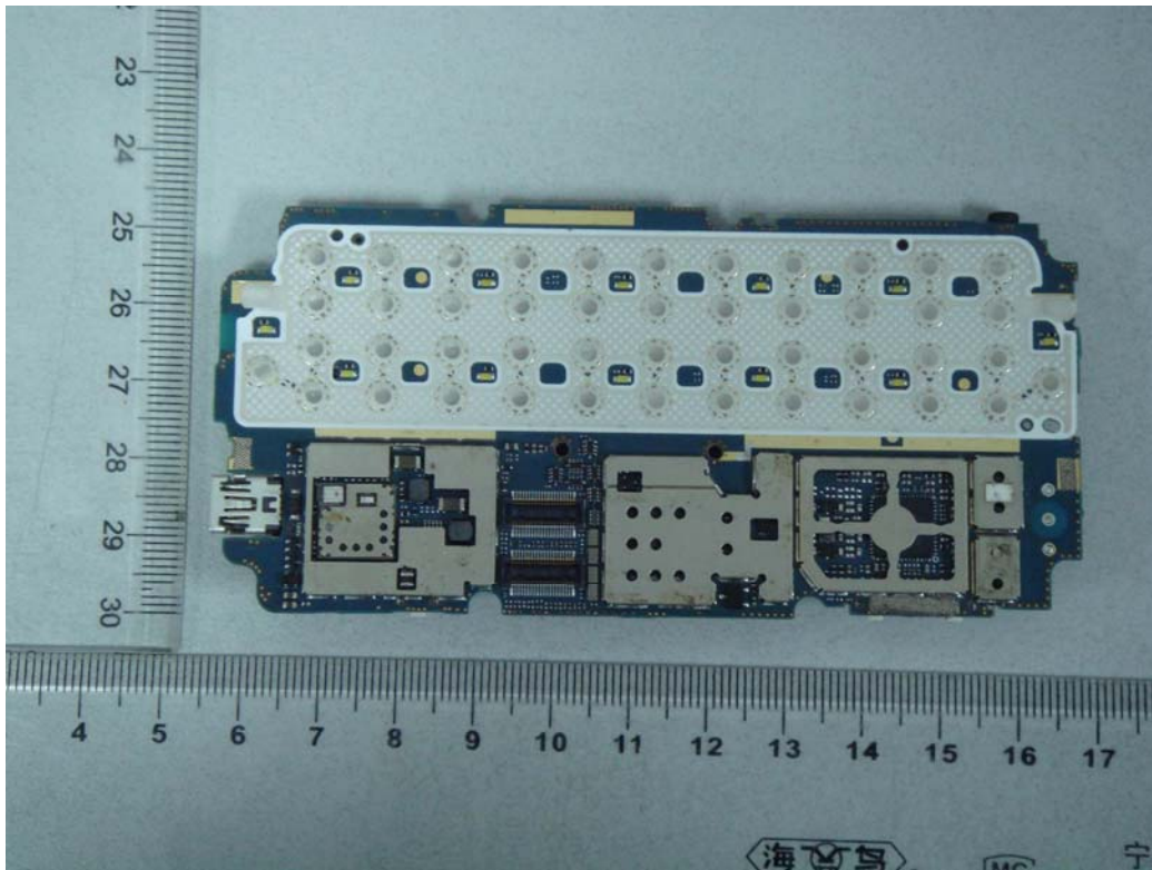
4. Main PCB without shielding(B)
