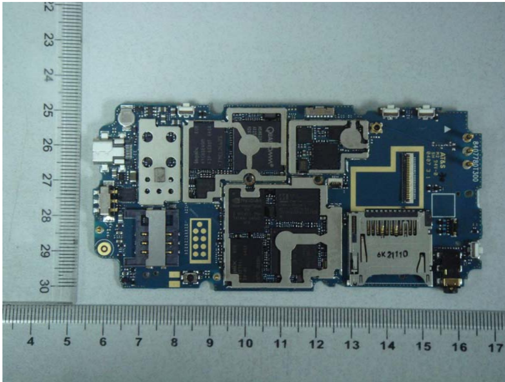
3. Main PCB without shielding(A)
