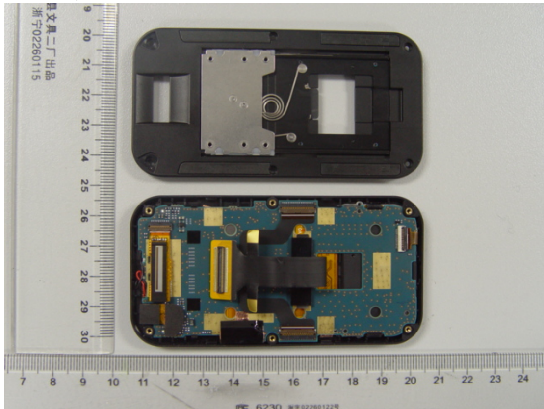
Front housing and slide PCB(1)
