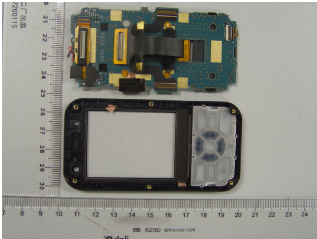
Front housing and slide PCB(2)
