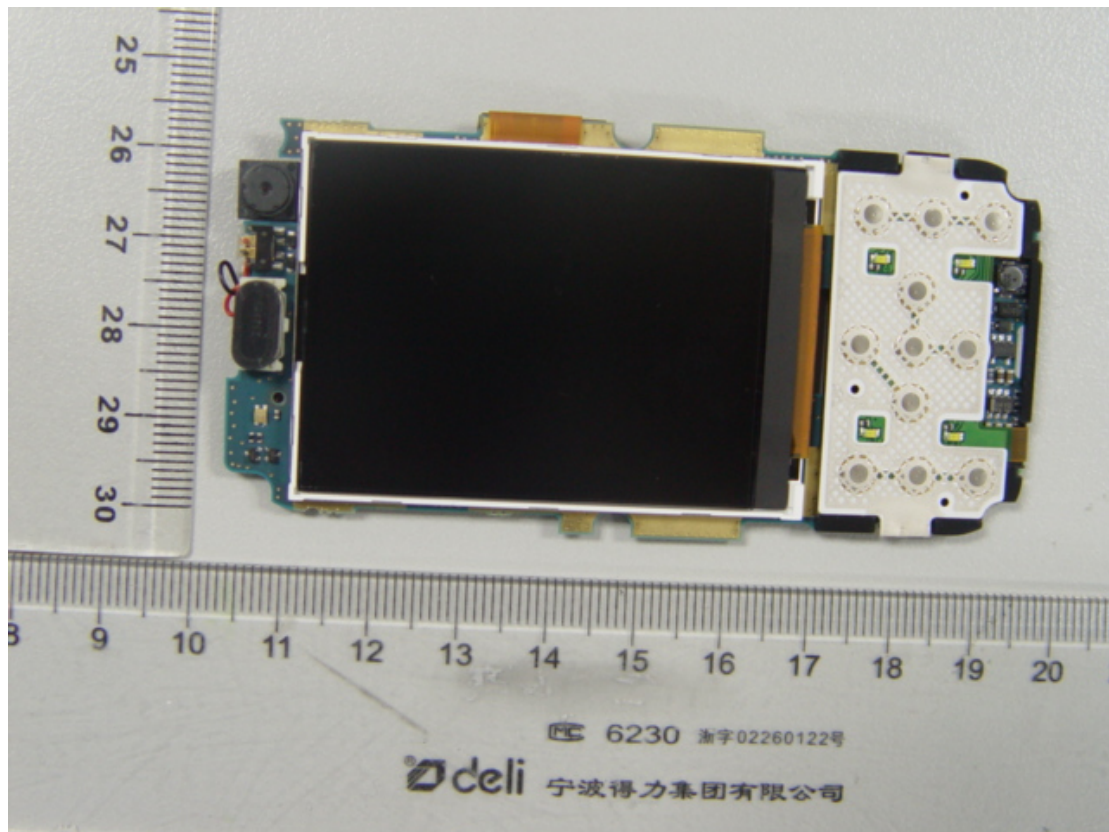
Slide PCB with LCD
