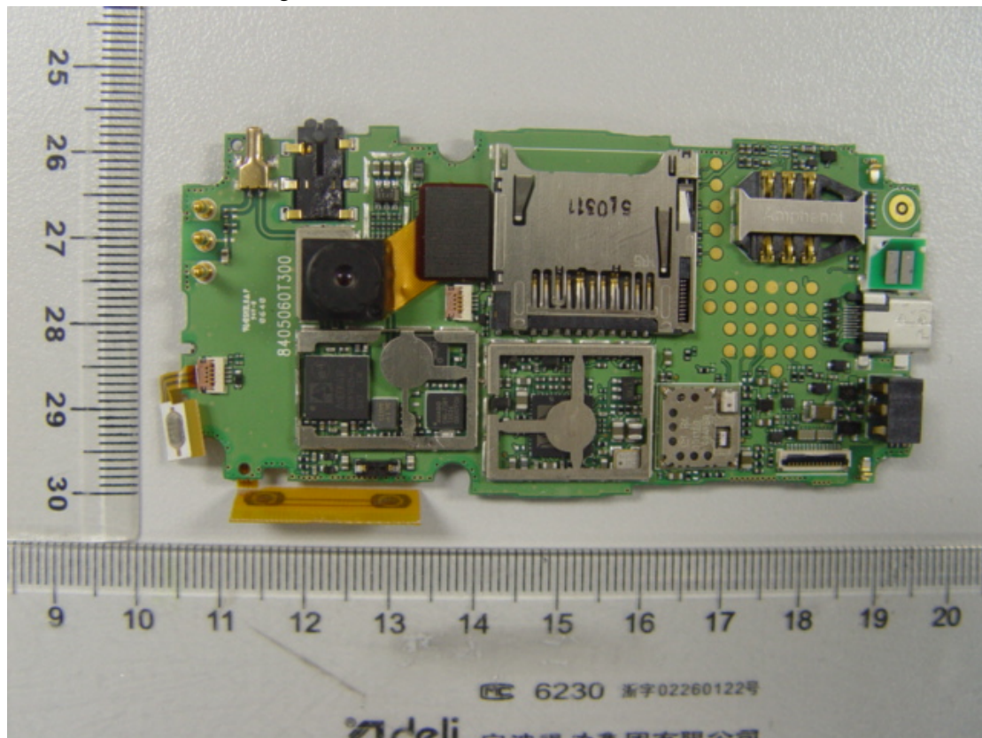
Main PCB without shielding(A)
