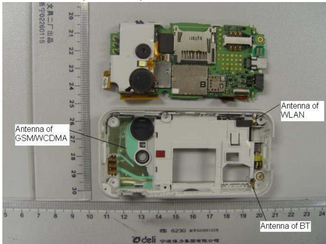
Main PCB with shielding and rear housing
