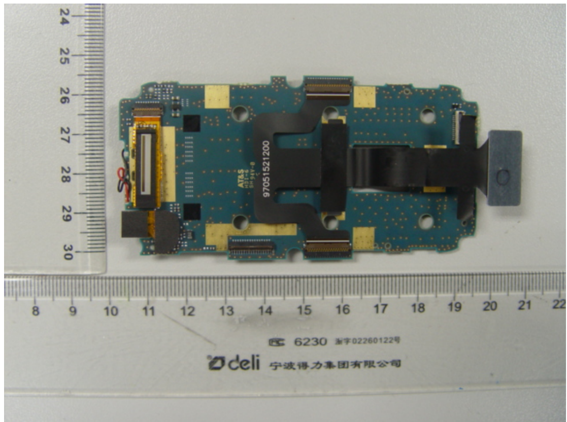
Slide PCB(A)
