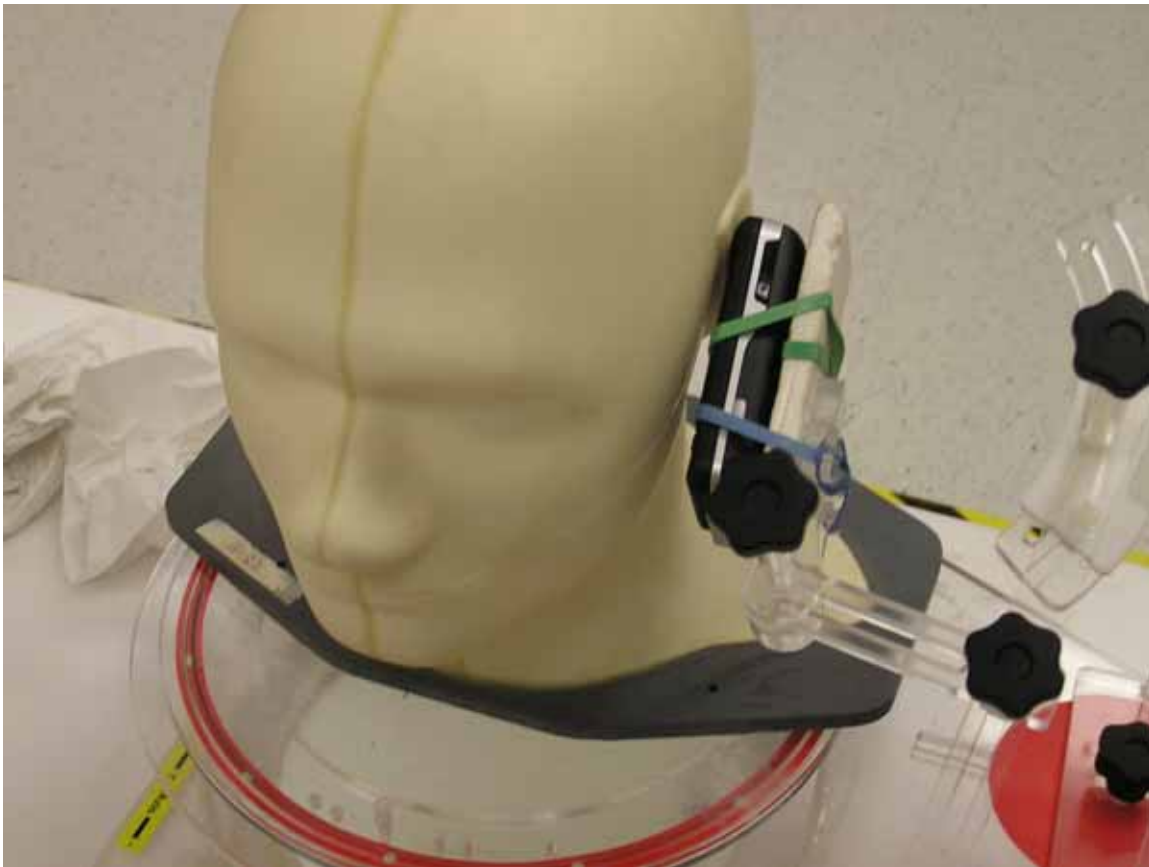
Photo 6: Left tilt slider closed
