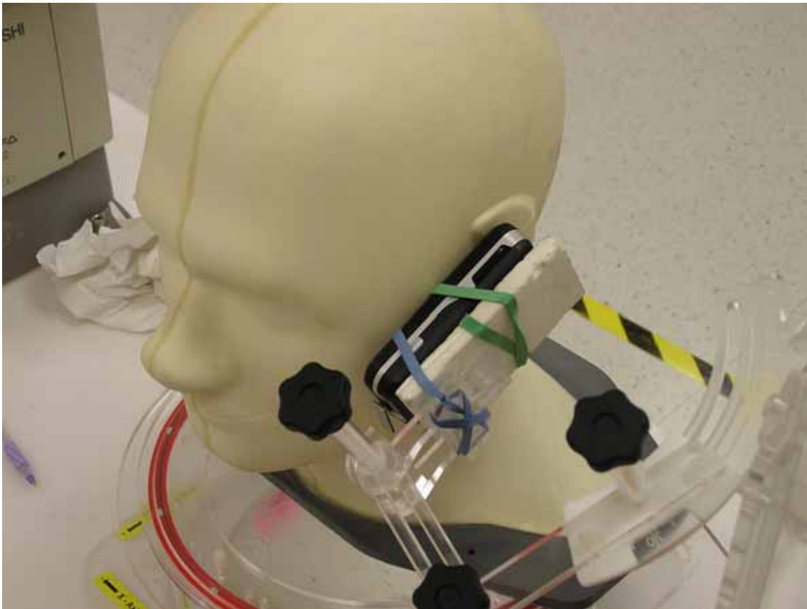
Photo 5: Left touch slider closed
