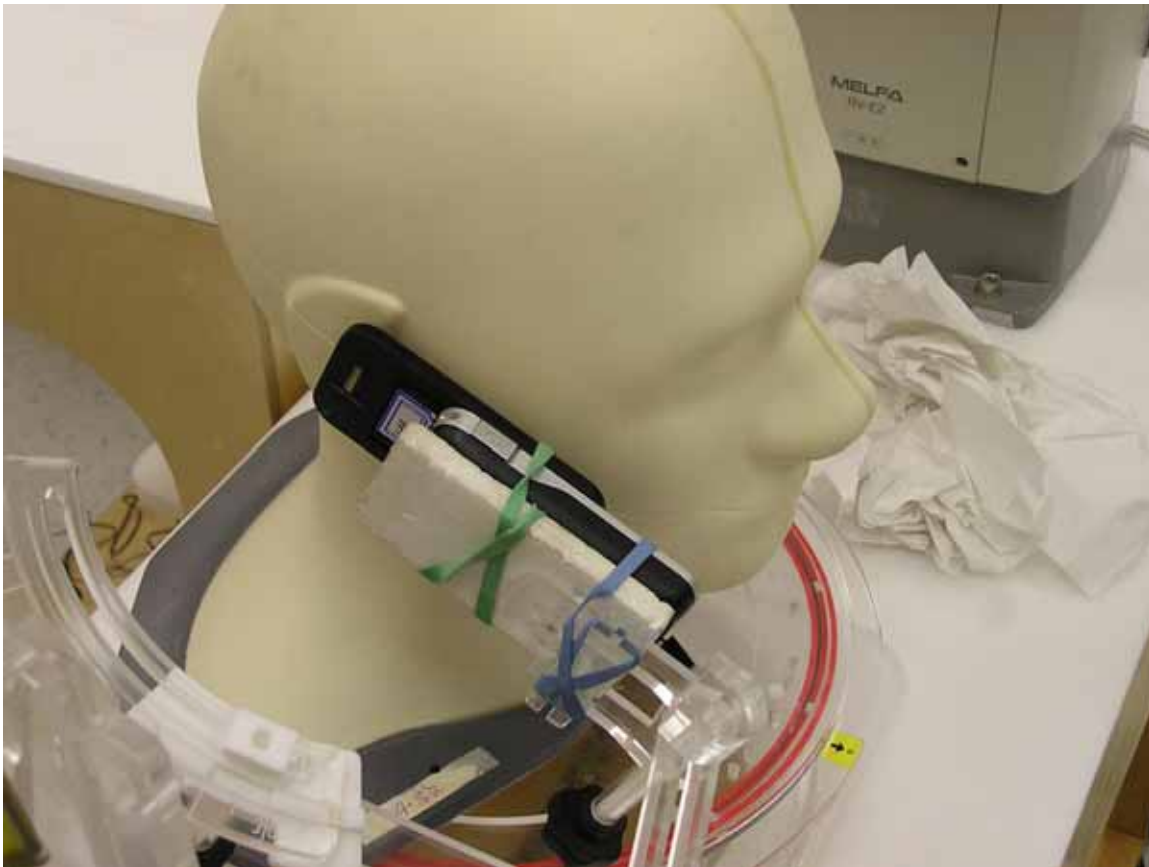
Photo 3: Right touch slider open
