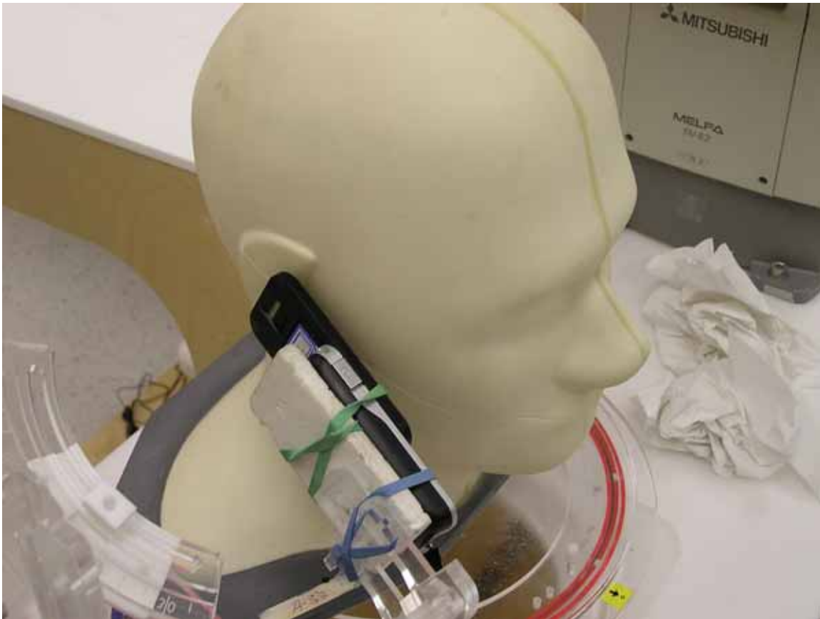
Photo 4: Right tilt slider open
