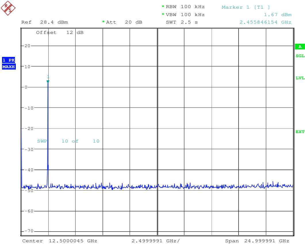
Plot 3: (DSSS)
