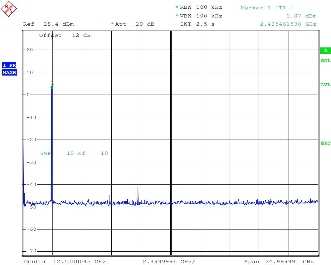
Plot 5: (OFDM)
