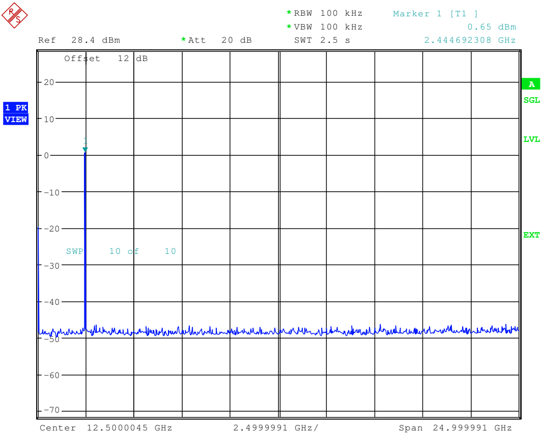
Plot 2: (DSSS)
