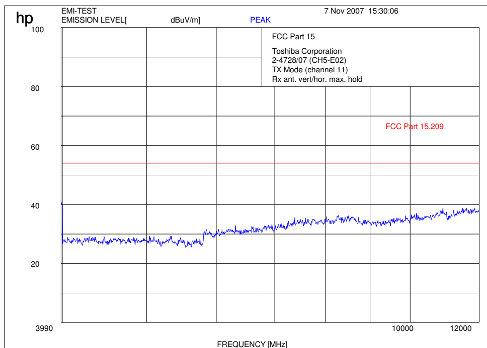
Plot 10: 4 - 12 GHz (highest channel) (b Mode – 1Mbps)
