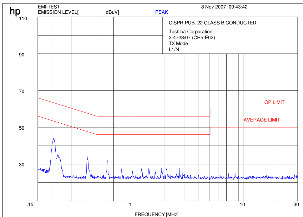
Plot 1: CISPR 22 – OFDM Mode
