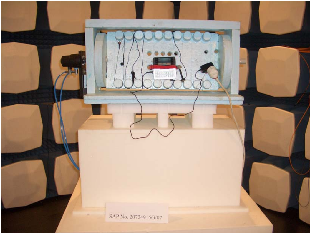
Photograph 6: Measurements in the anechoic chamber
