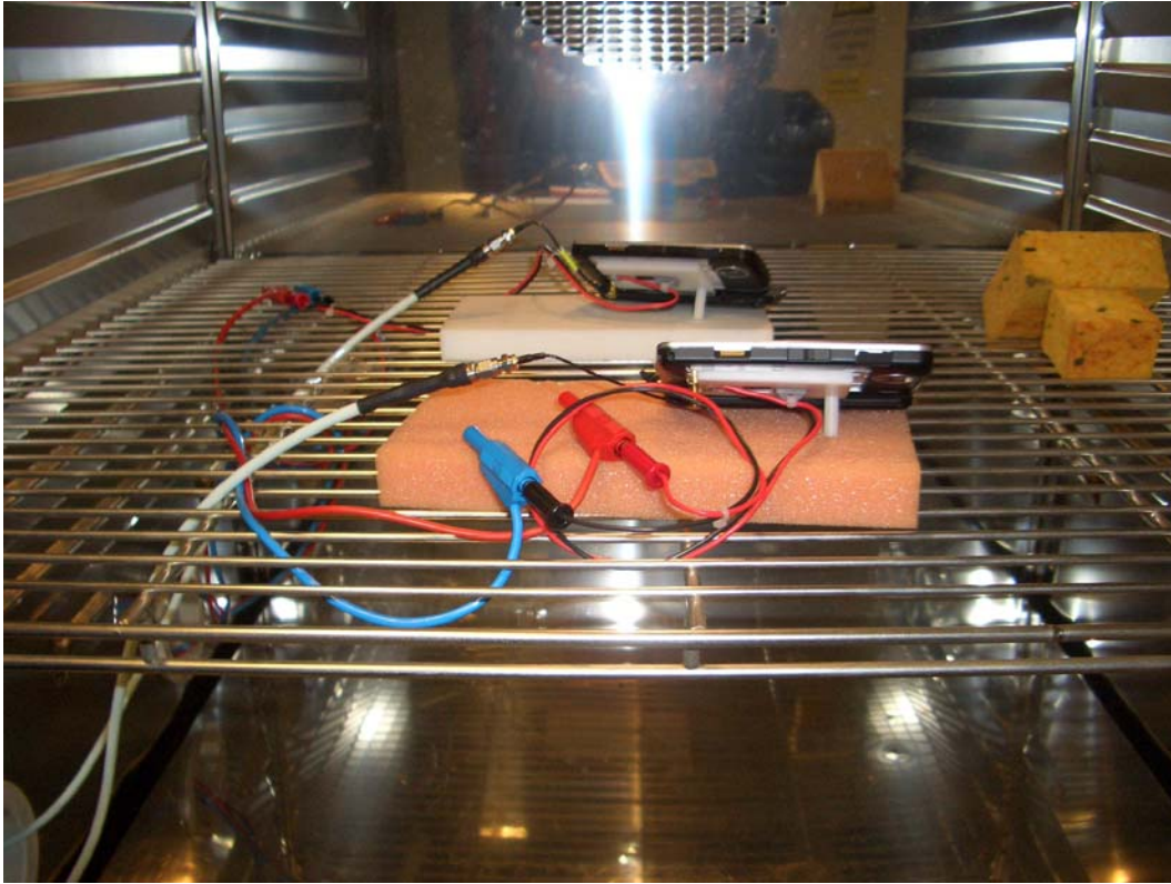
Photograph 7: Measurements in the climatic chamber
