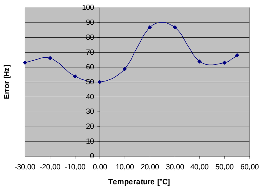
EGPRS Frequency error / Channel 810
