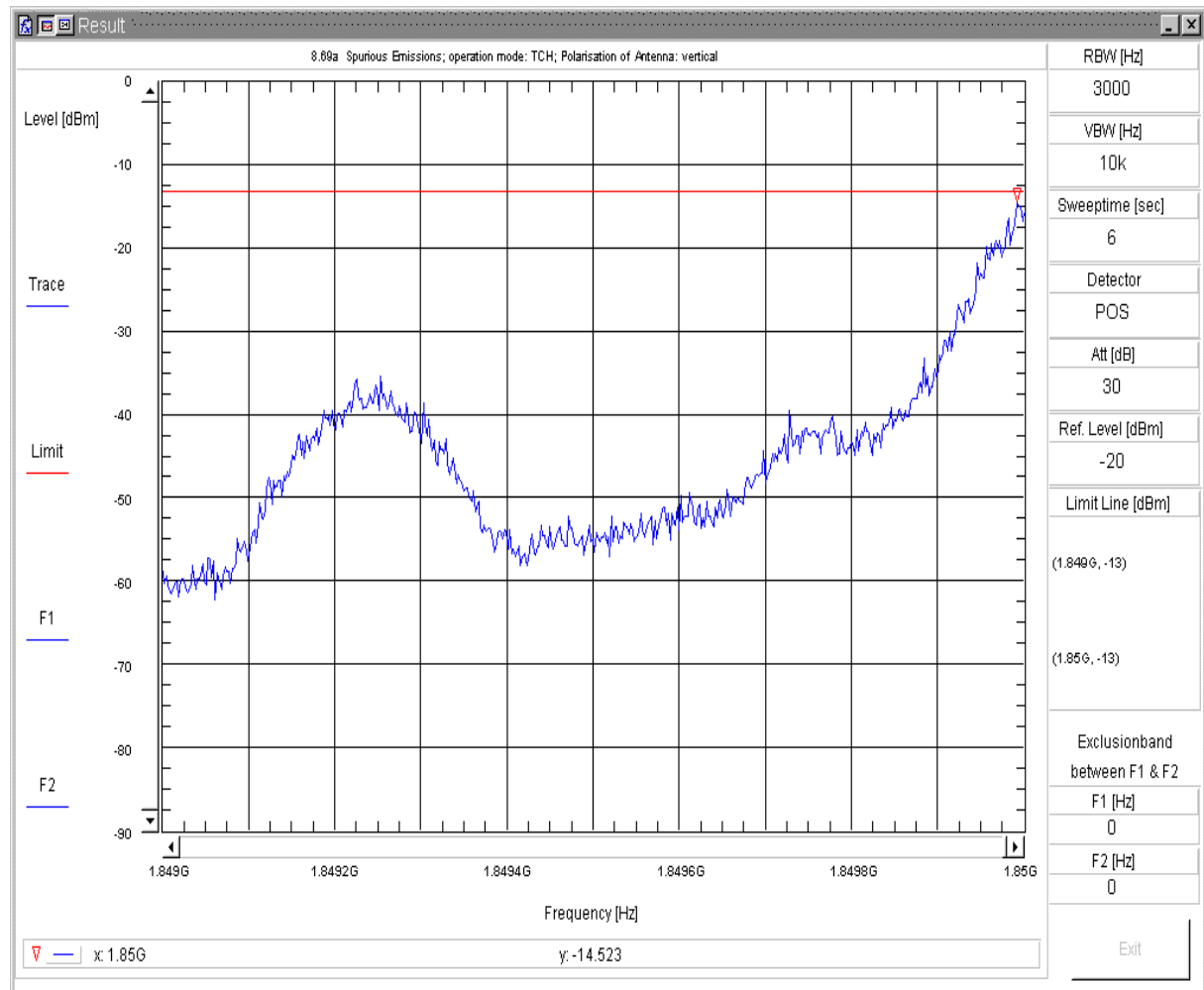
8.69a Radiated Spurious Emission
