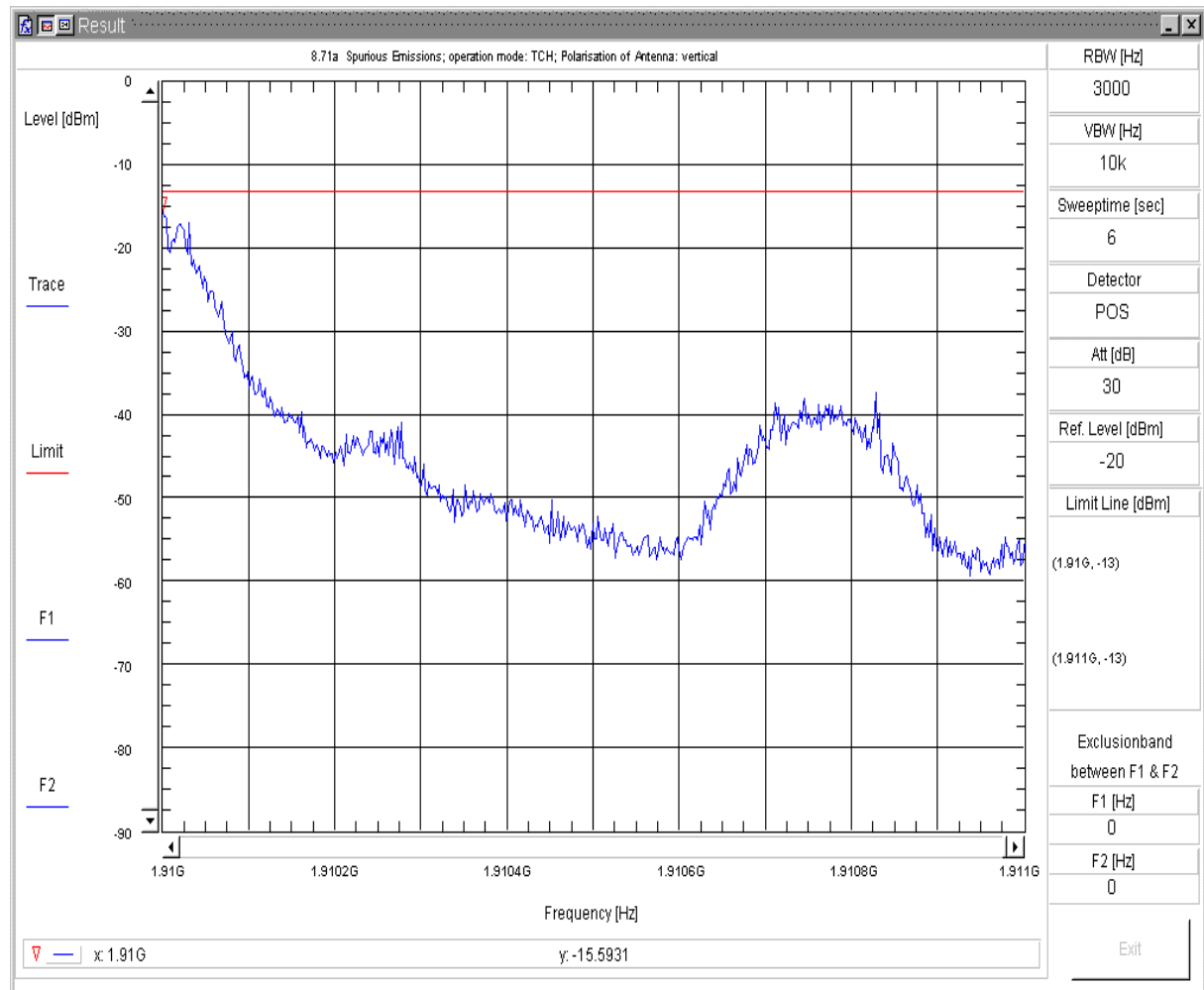
8.71a Radiated Spurious Emission
