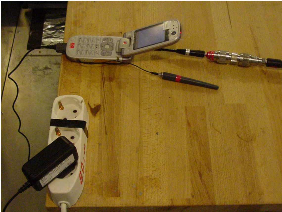
Photo 5: Setup for the test "Conducted emissions (AC power line)"
