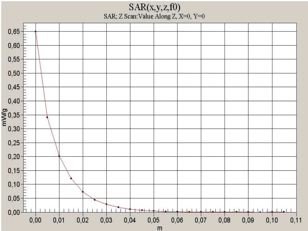
Photo 27: Z-axis scans 1900 MHz head
