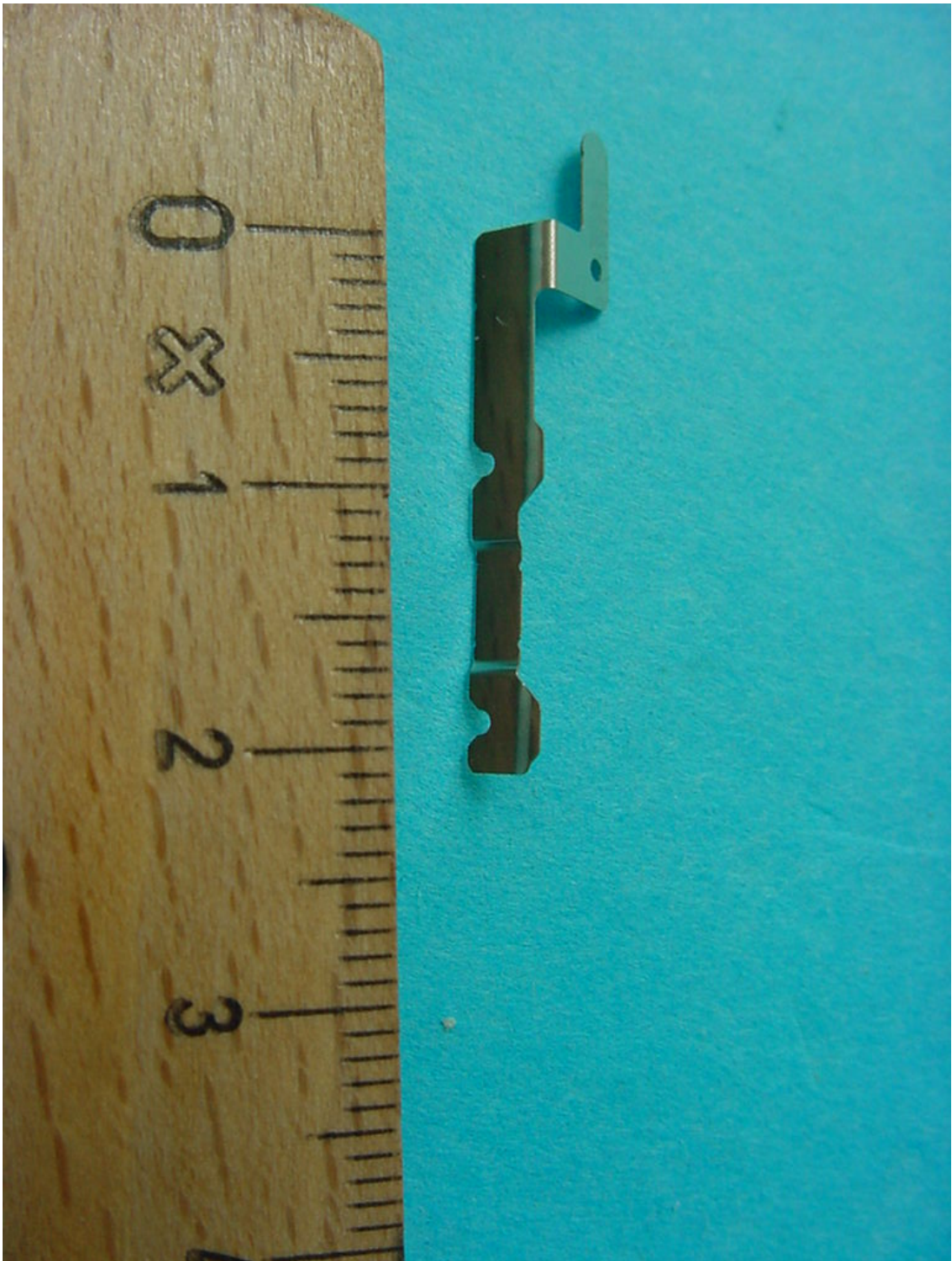
Photo 2: 2.4 GHz antenna
